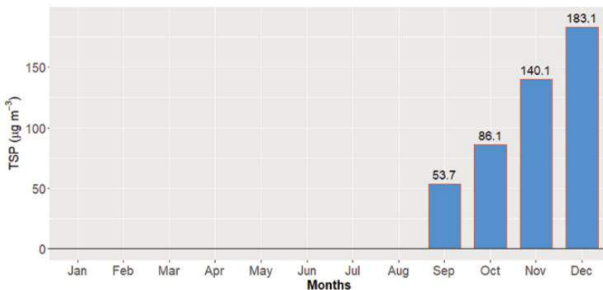
Figure 126: Monthly average of TSP for Shankhapark Station
