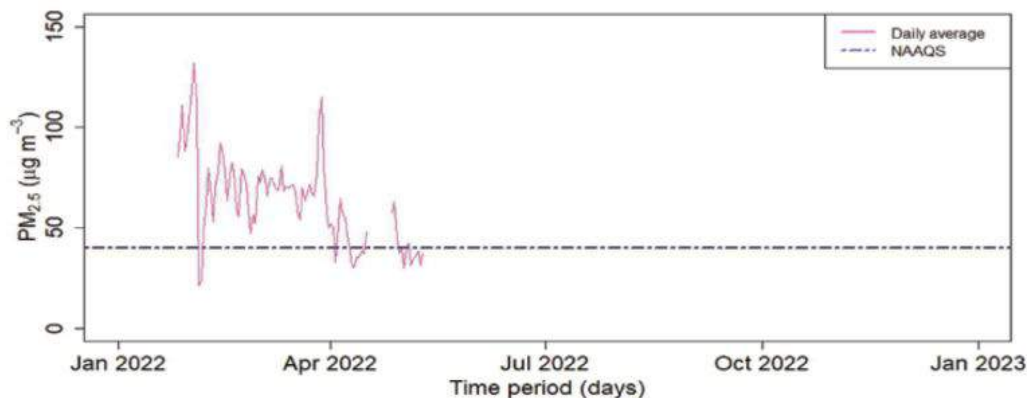
Figure 29: Daily average of PM 2.5 for Bharatpur Station
