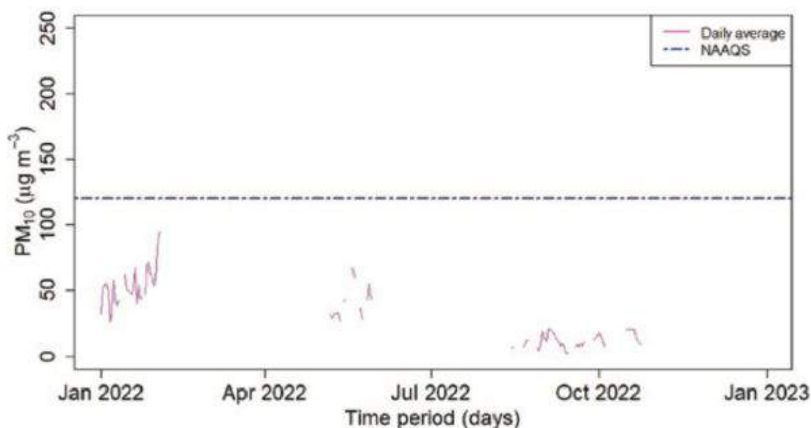
Figure 162: Daily average of PM 10 for Dang Station
