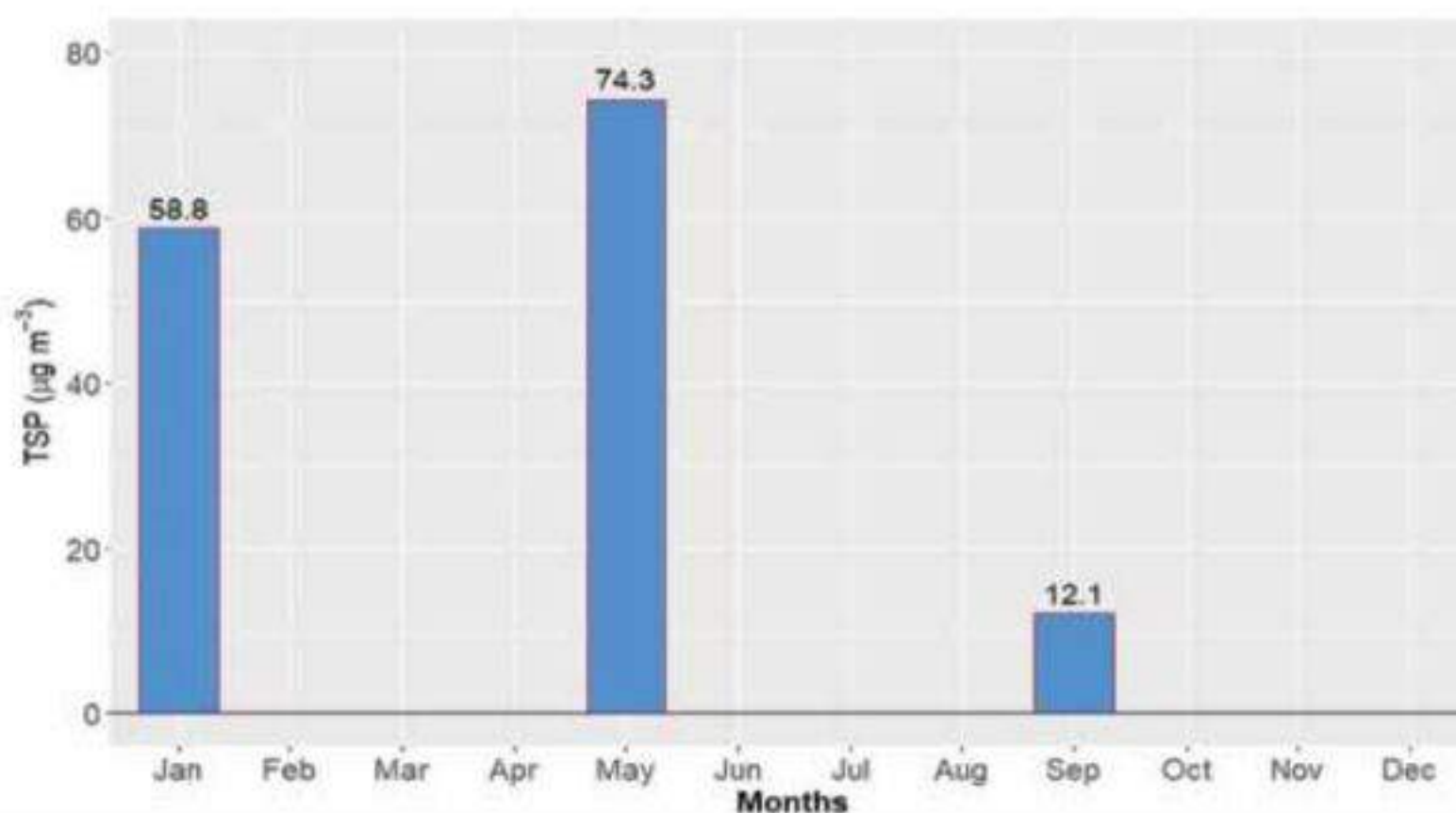
Figure 170: Monthly average of TSP for Dang Station
