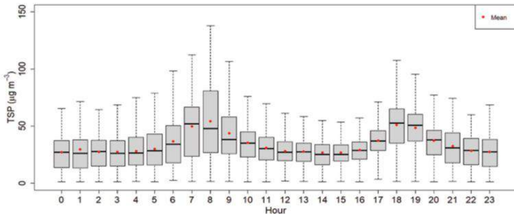
Figure 233: Diurnal variation of TSP for Surkhet Station
