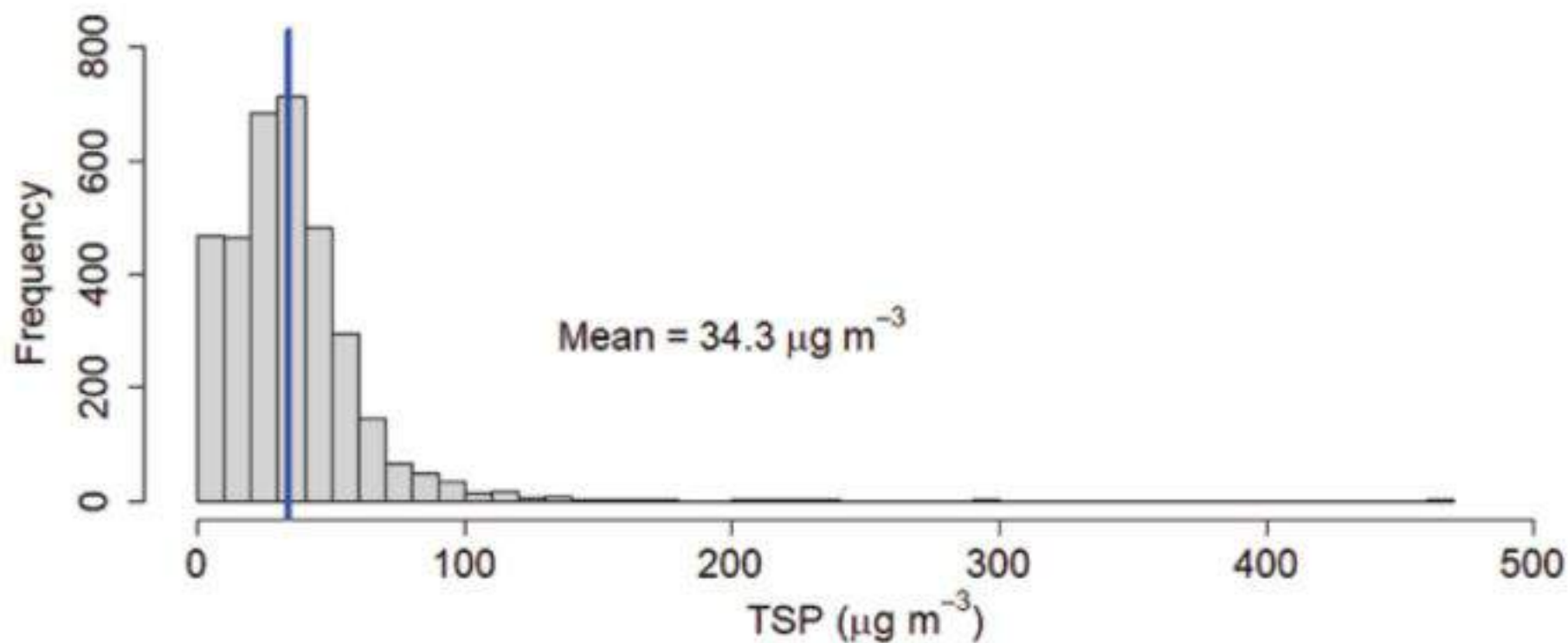
Figure 232: Histogram of TSP for Surkhet Station
