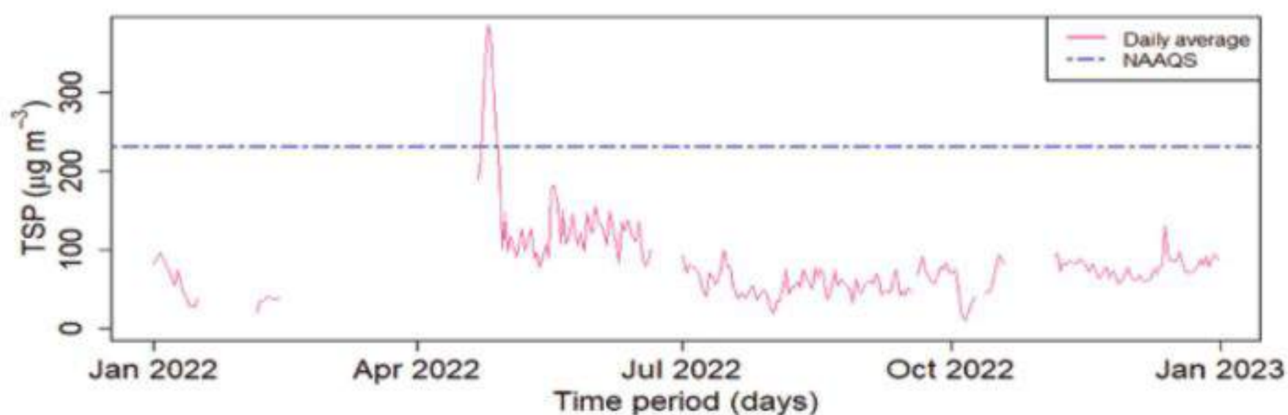
Figure 103: Daily average of TSP for Ratnapark Station
