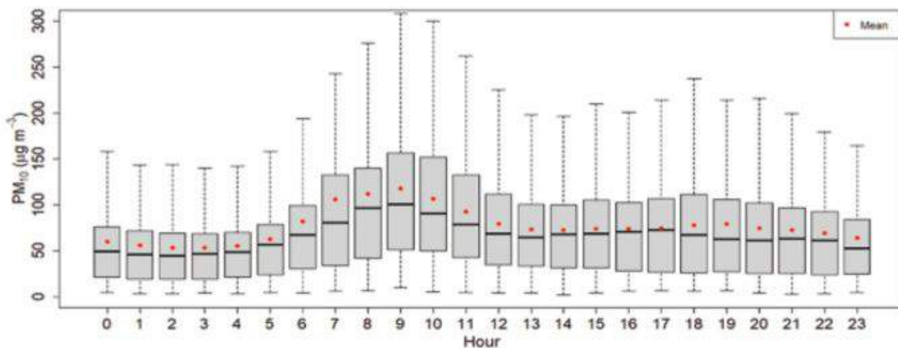
Figure 79: Diurnal variation of PM 10 for Khumaltar Station
