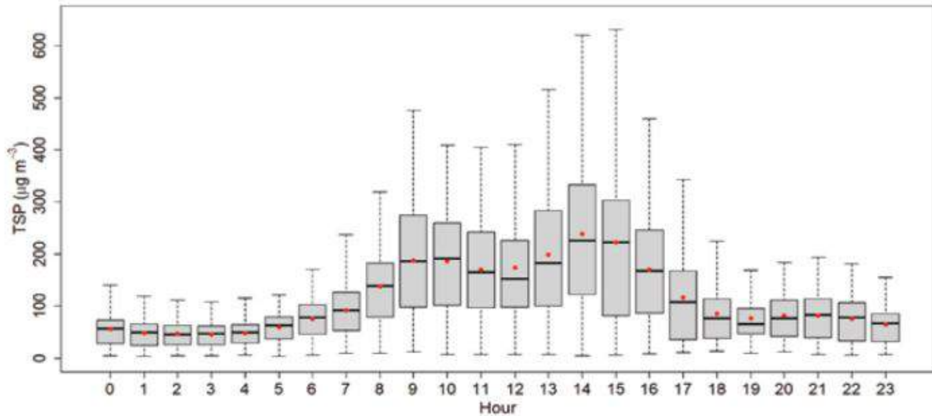
Figure 123: Diurnal variation of TSP for Shankhapark Station
