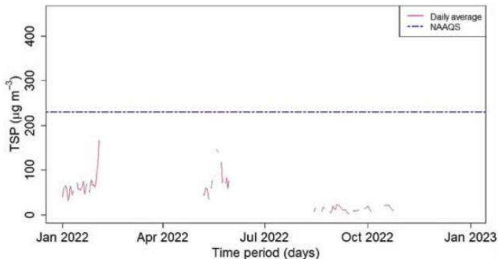
Figure 169: Daily average of TSP for Dang Station
