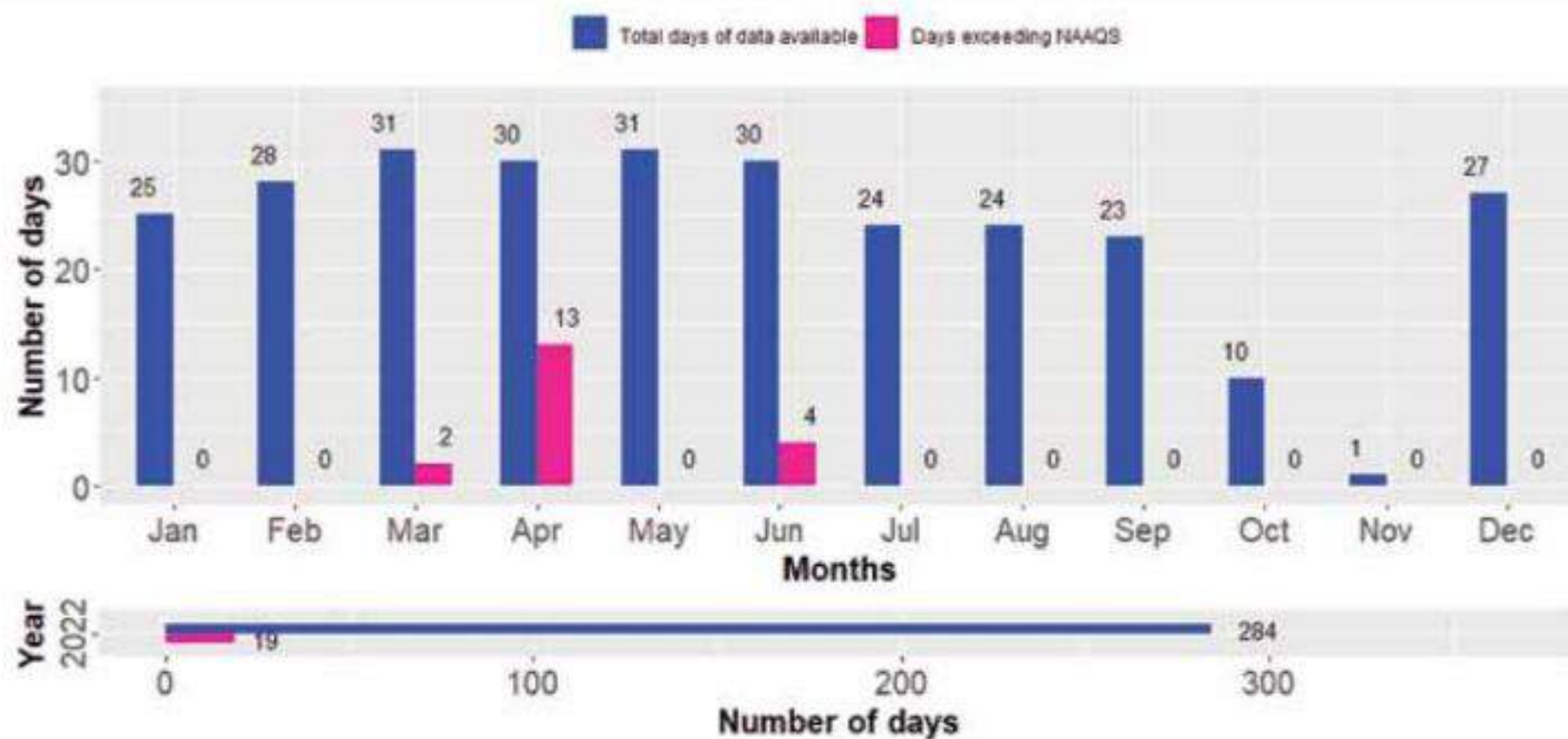
Figure 201: Compliance status of PM 2.5 for Rara Station
