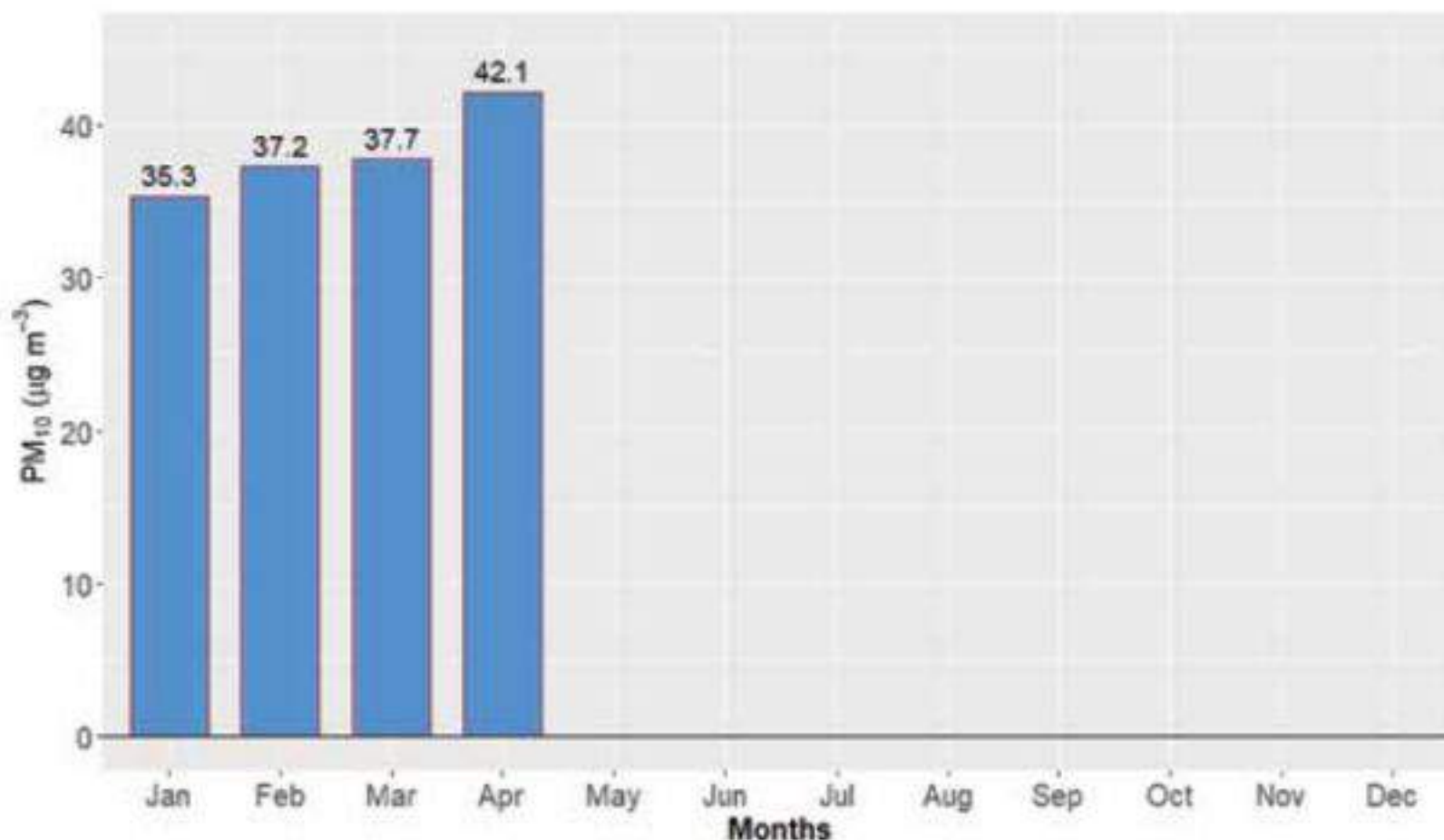
Figure 229: Monthly average of PM 10 for Surkhet Station
