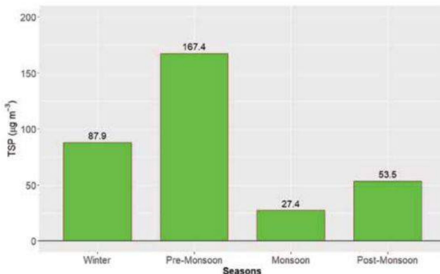
Figure 24: Seasonal average of TSP for Dhankuta Station
