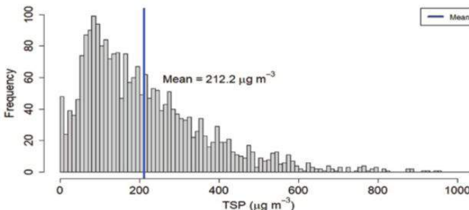
Figure 41: Histogram of TSP for Bharatpur Station
