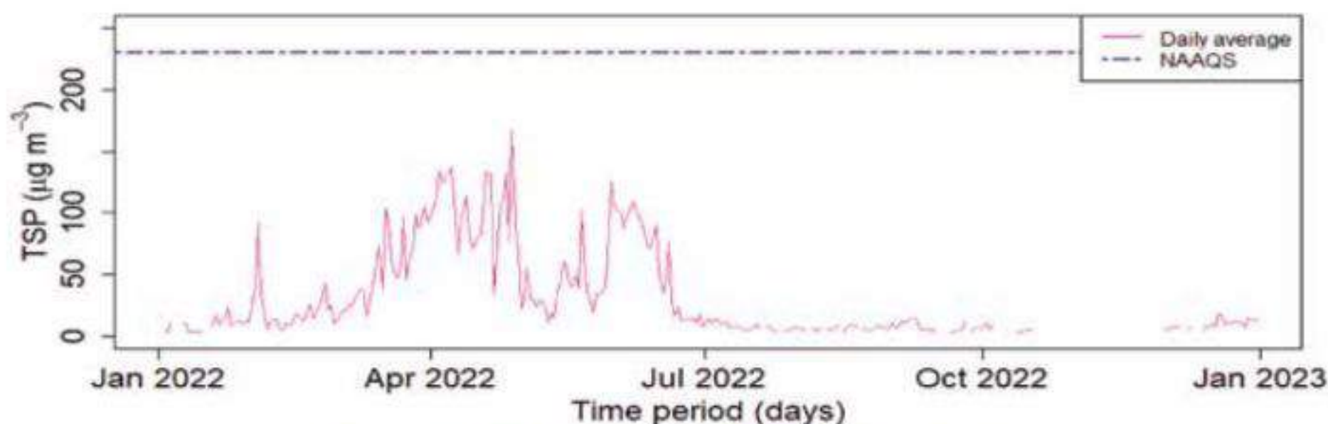
Figure 213: Daily average of TSP for Rara Station
