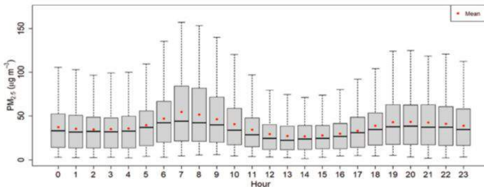
Figure 71: Diurnal variation of PM 2.5 for Khumaltar Station
