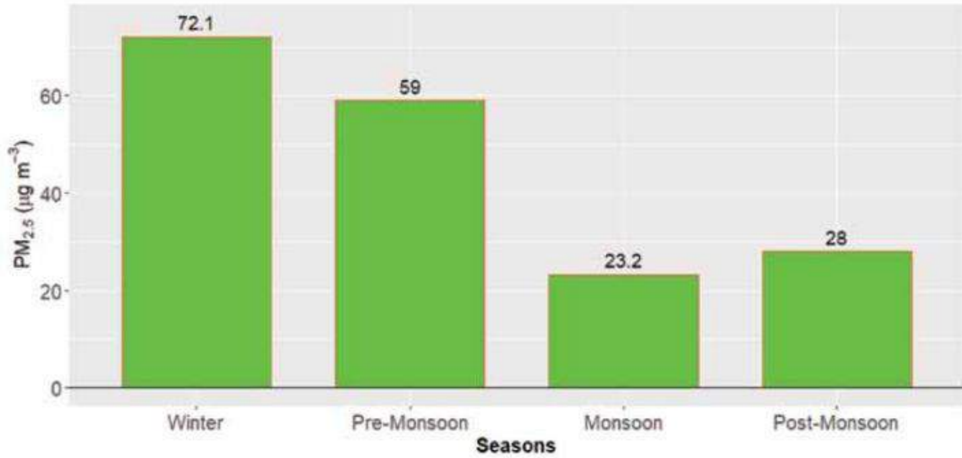
Figure 134: Seasonal average of PM 2.5 for Kirtipur Station
