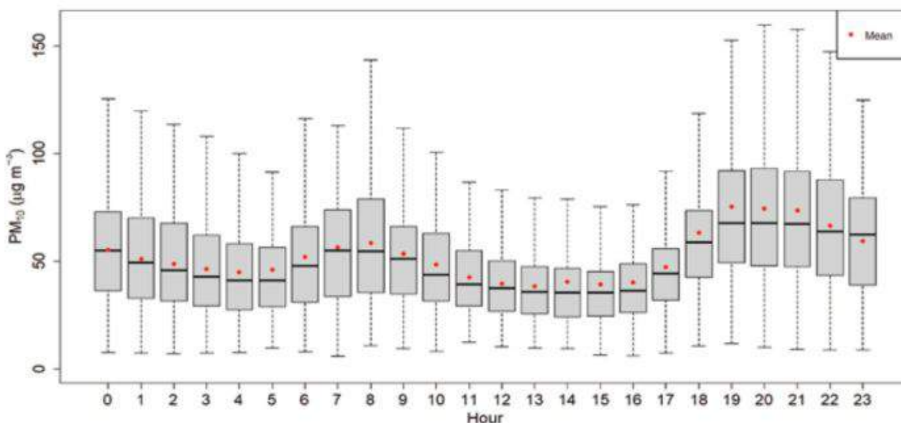
Figure 182: Diurnal variation of PM 10 for Nepalgunj Station
