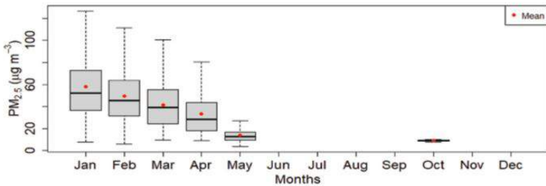
Figure 175: Monthly variation of PM_{2.5} for Nepalgunj Station
