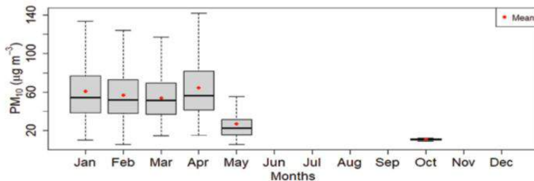
Figure 183: Monthly variation of PM_{10} for Nepalgunj Station
