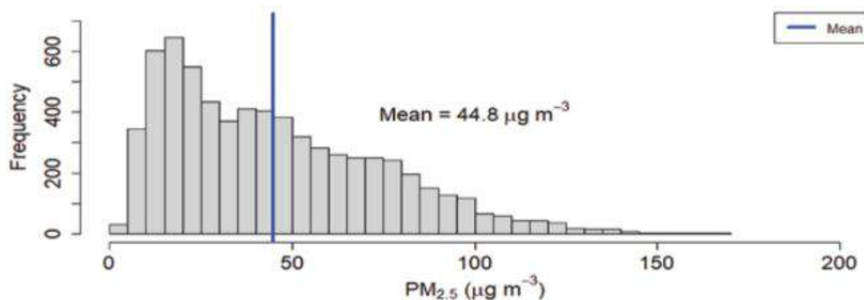
Figure 129: Histogram of PM_{2.5} for Kirtipur Station
