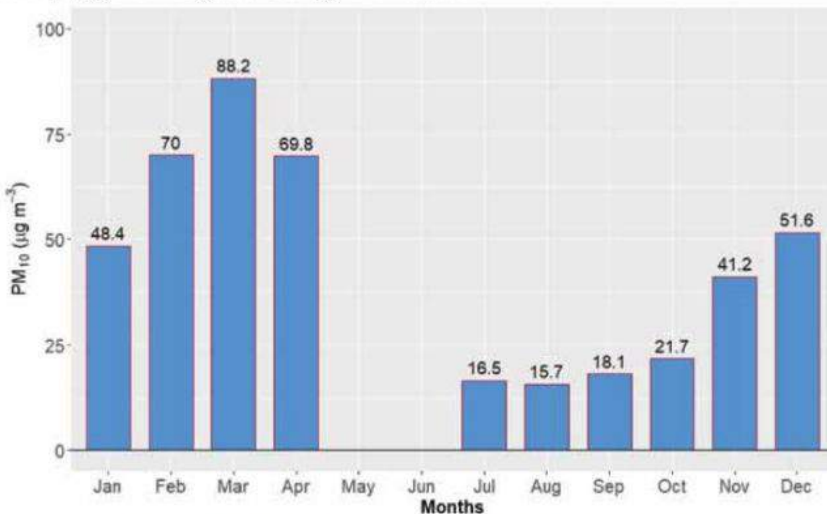
Figure 16: Monthly average of PM 10 for Dhankuta Station
