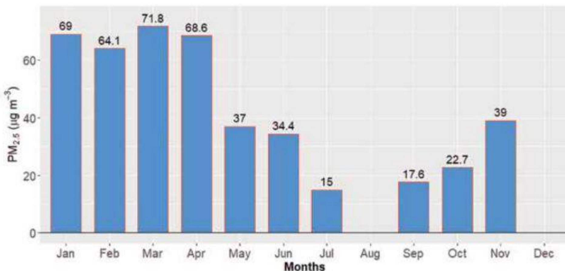
Figure 133: Monthly average of PM 2.5 for Kirtipur Station
