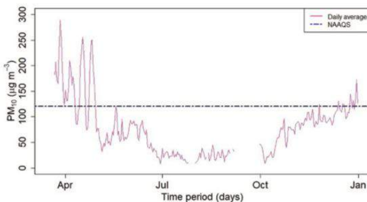
Figure 81: Daily average of PM_{10} for Khumaltar Station
