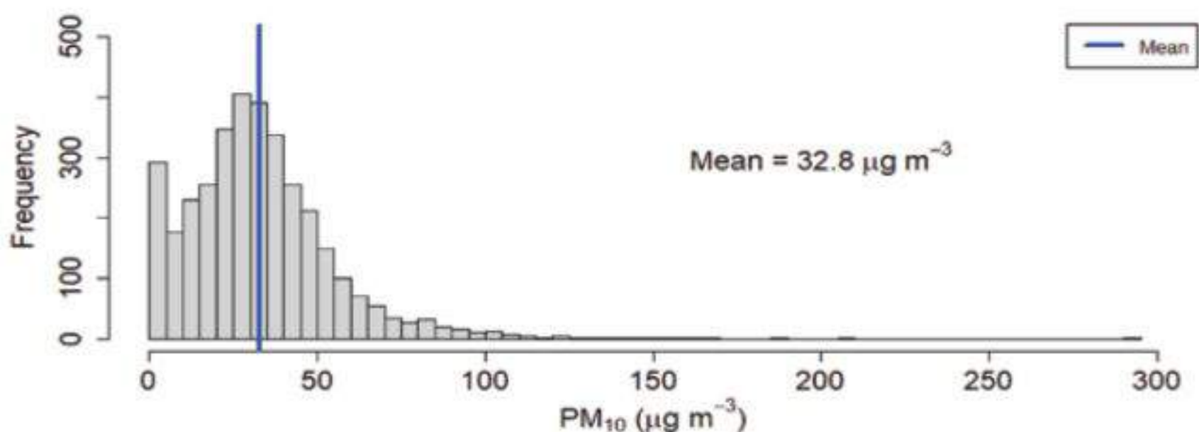
Figure 225: Histogram of PM 10 for Surkhet Station
