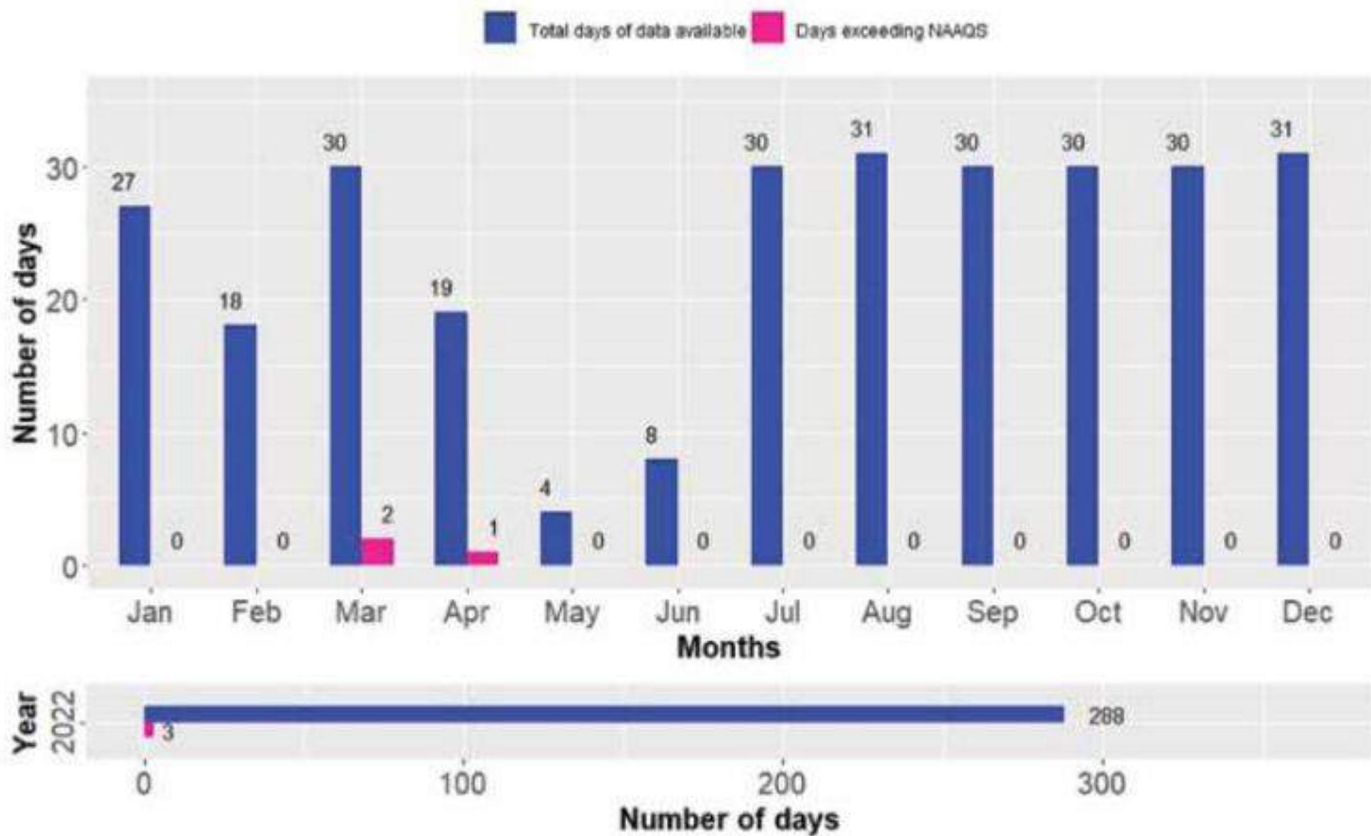
Figure 18: Compliance status of PM 10 for Dhankuta Station
