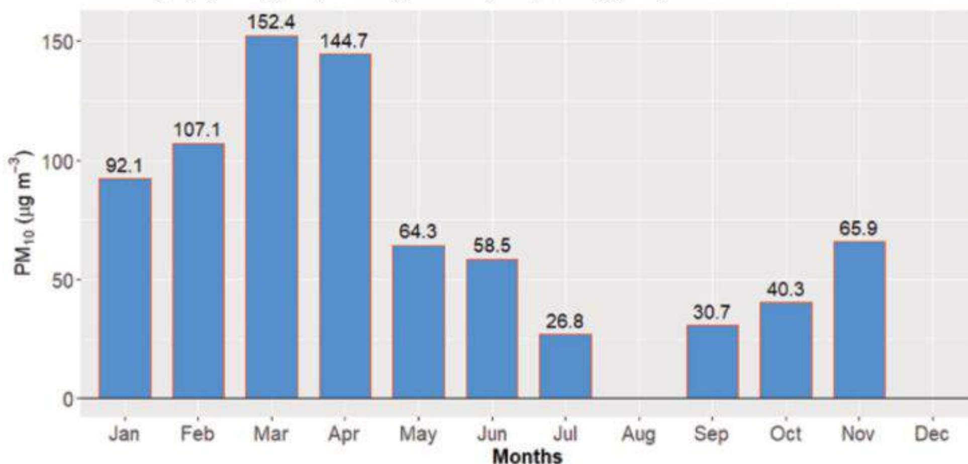
Figure 141: Monthly average of PM 10 for Kirtipur Station
