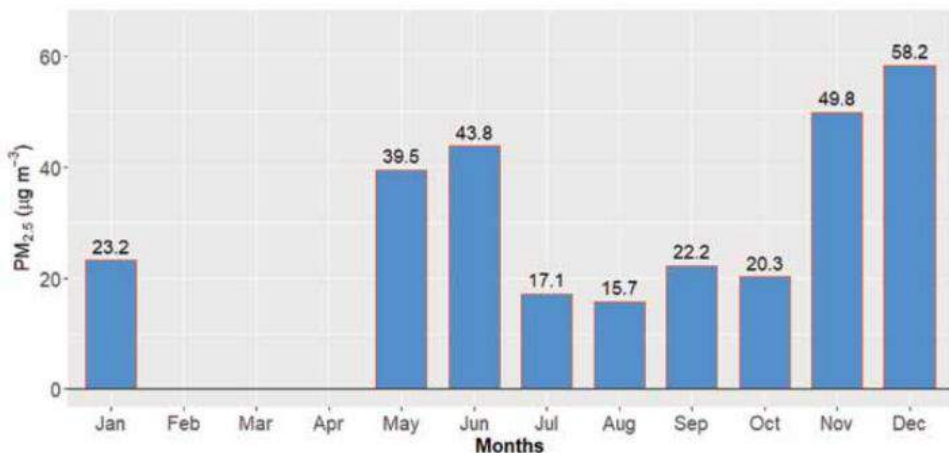
Figure 89: Monthly average of PM_{2.5} for Ratnapark Station
