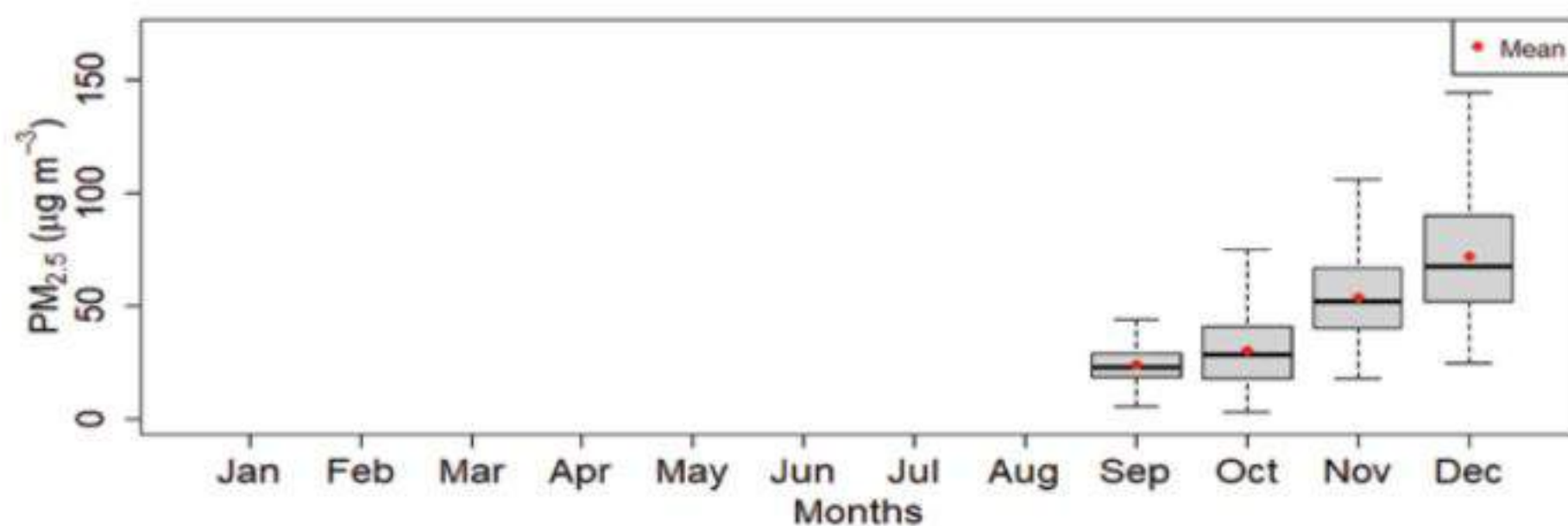
Figure 109: Monthly variation of PM 2.5 for Shankhapark Station
