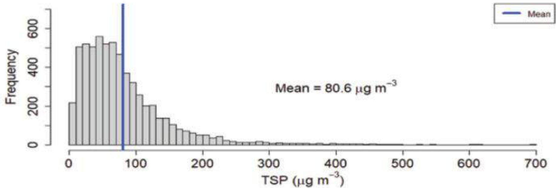
Figure 100: Histogram of TSP for Ratnapark Station
