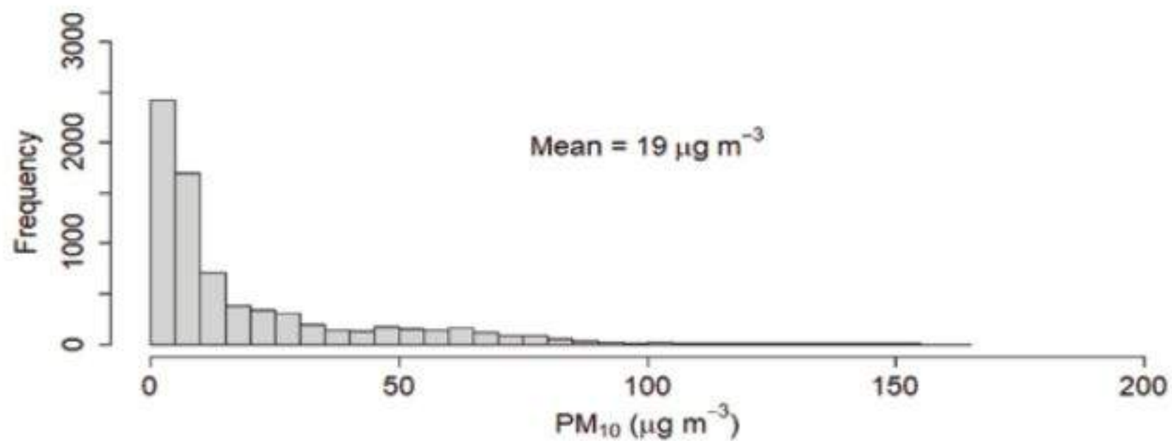
Figure 203: Histogram of PM 10 for Rara Station
