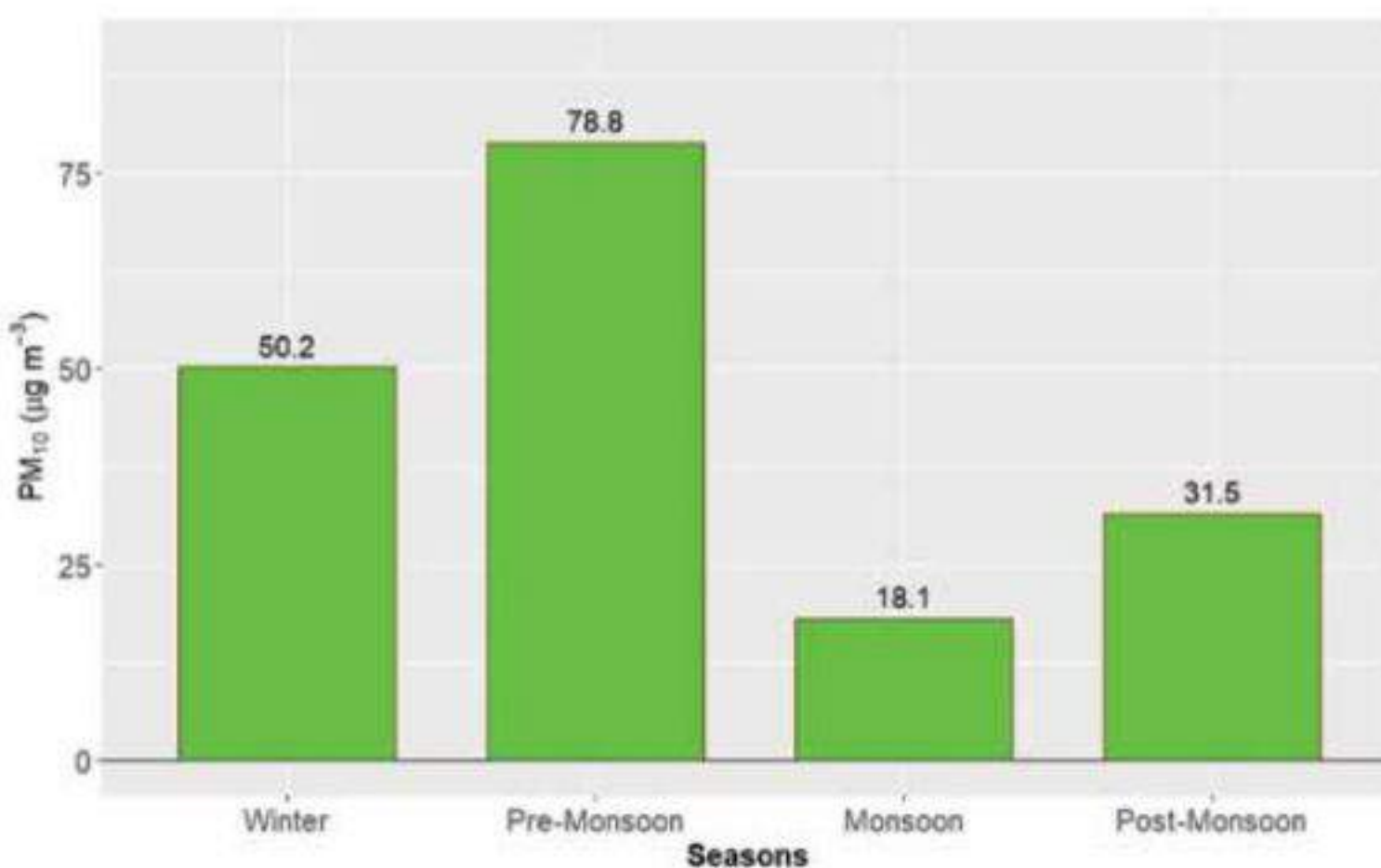
Figure 17: Seasonal average of PM 10 for Dhankuta Station
