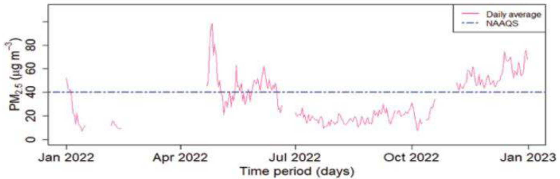
Figure 88: Daily average of PM_{2.5} for Ratnapark Station
