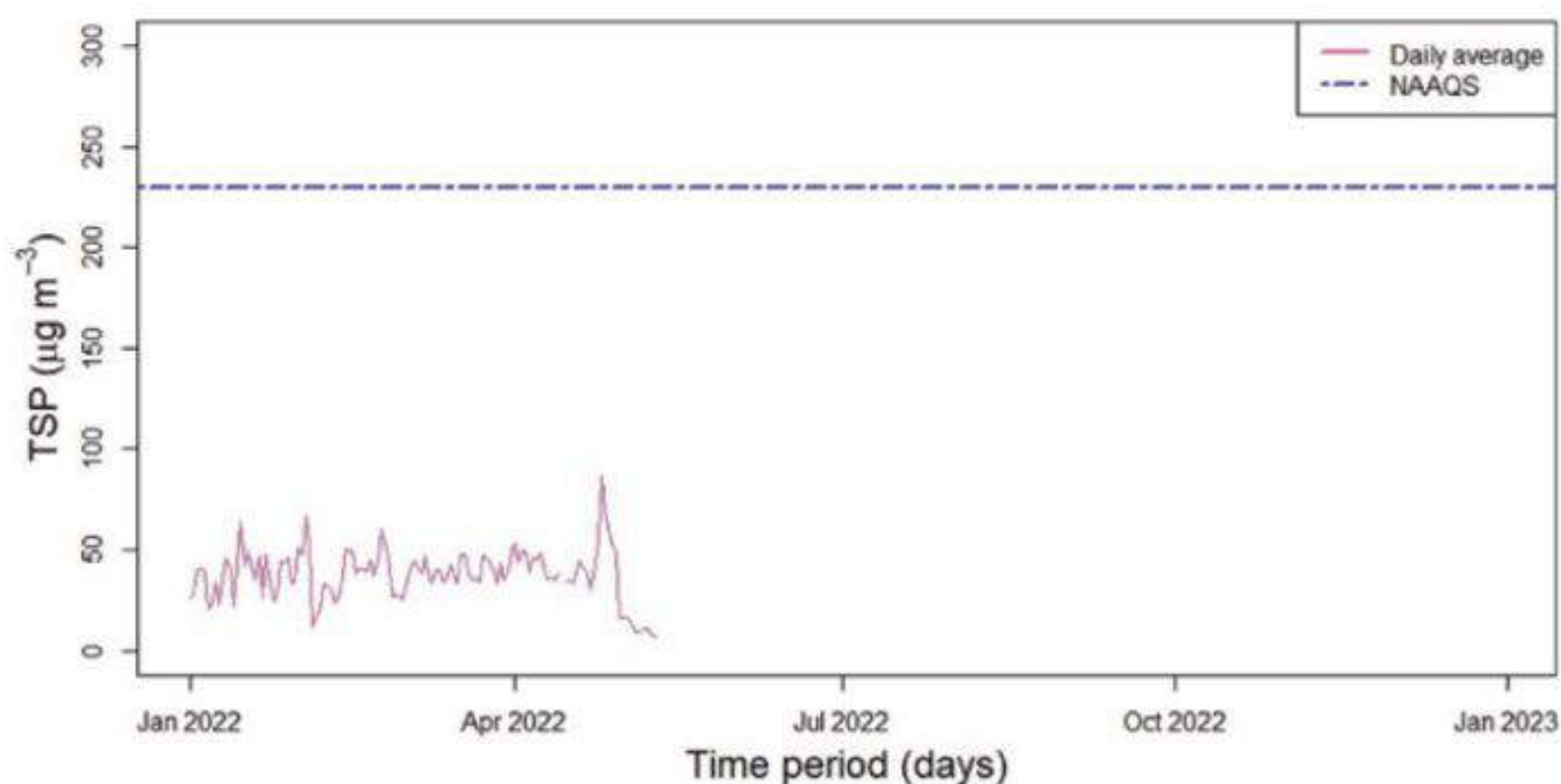
Figure 235: Daily average of TSP for Surkhet Station
