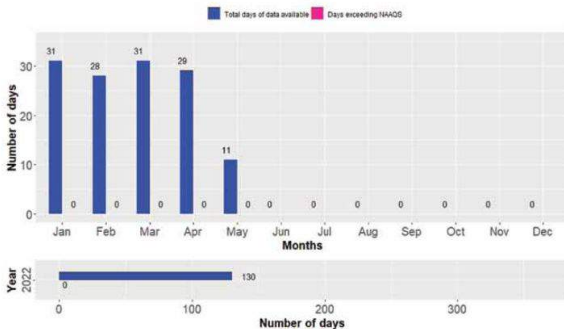
Figure 231: Compliance status of PM_{10} for Surkhet Station
