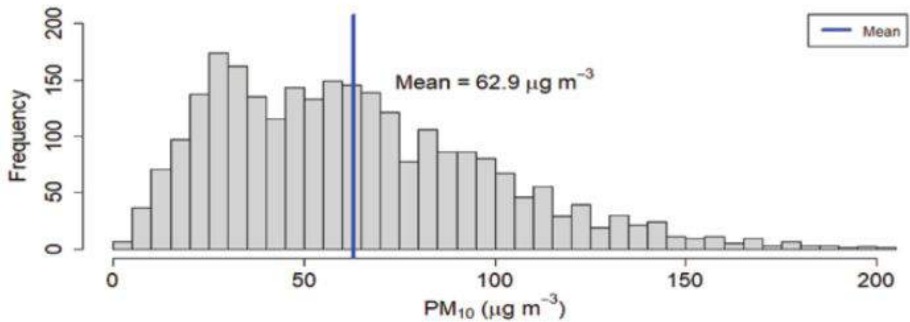
Figure 115: Histogram of PM_{10} for Shankhapark Station
