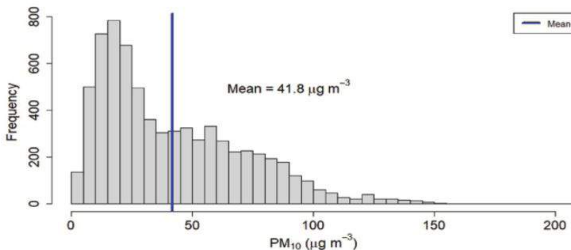
Figure 12: Histogram of PM 10 for Dhankuta Station
