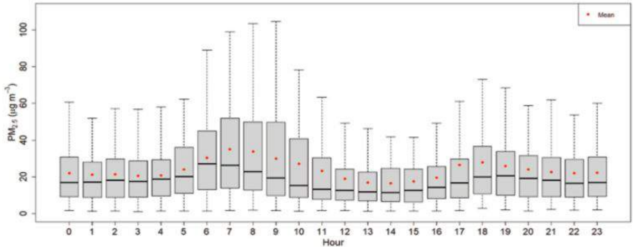
Figure 152: Diurnal variation of PM_{2.5} for Dang Station
