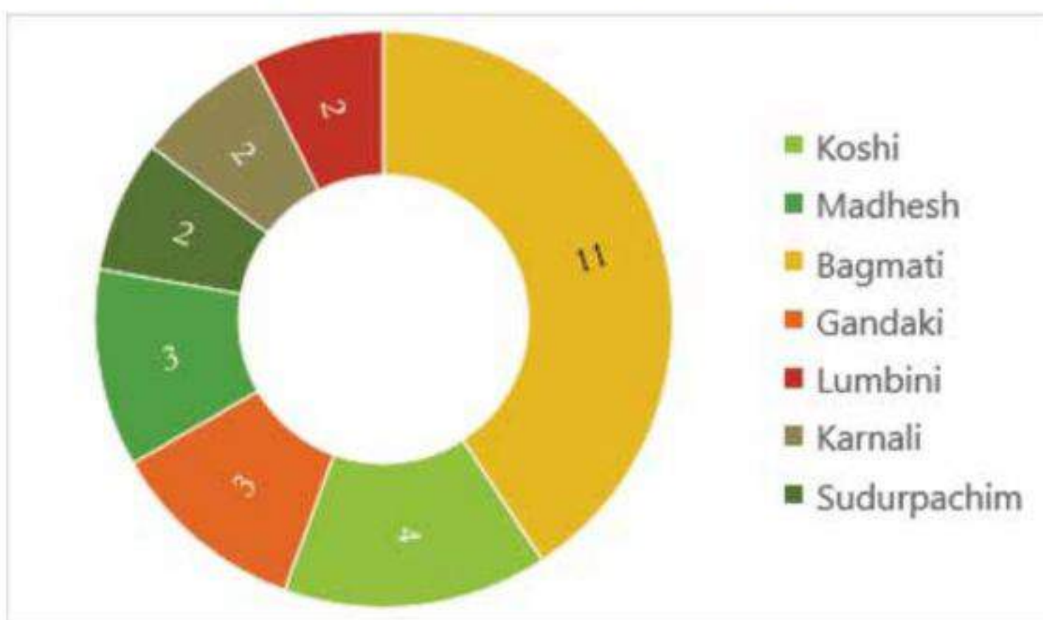
Figure 3: Provincial distribution of Air Quality Monitoring Stations
