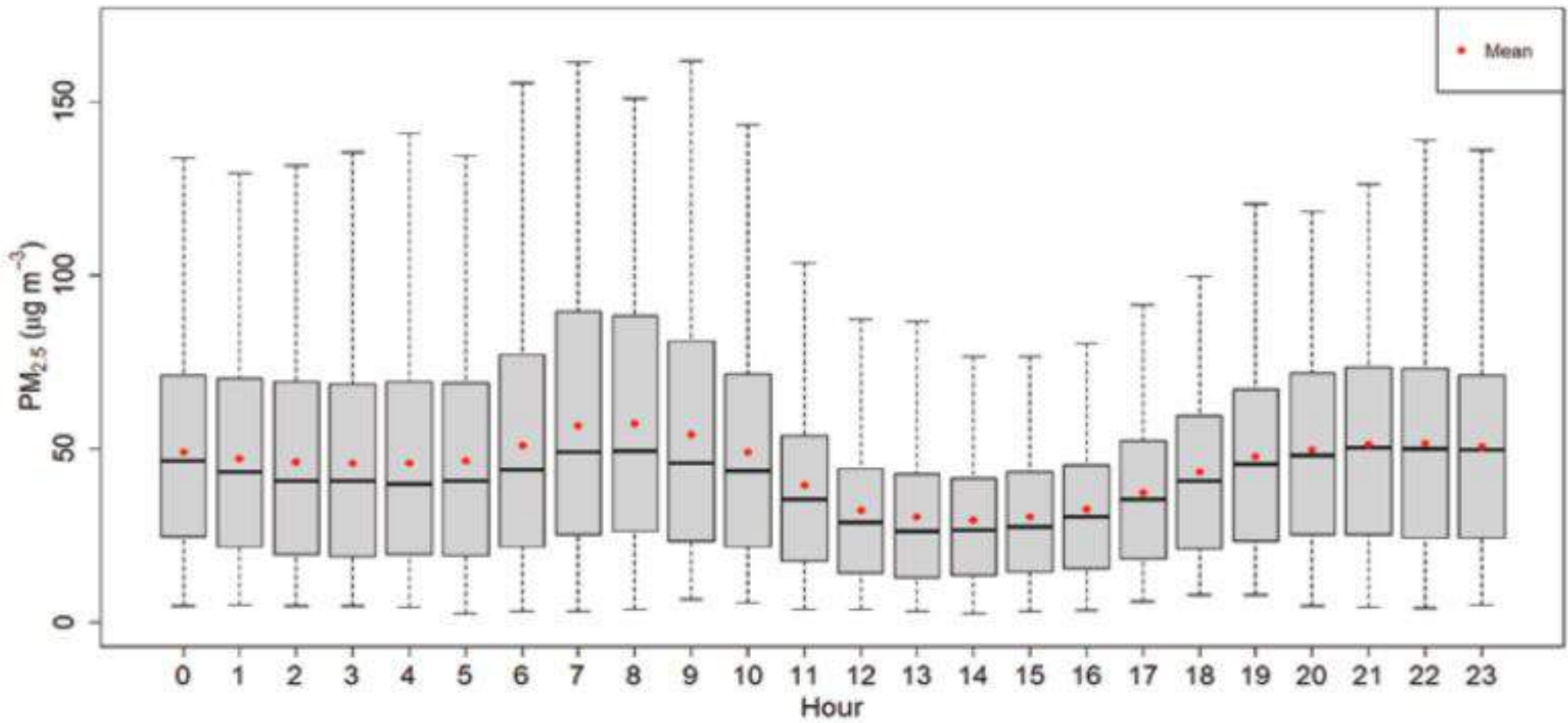
Figure 130: Diurnal variation of PM_{2.5} for Kirtipur Station
