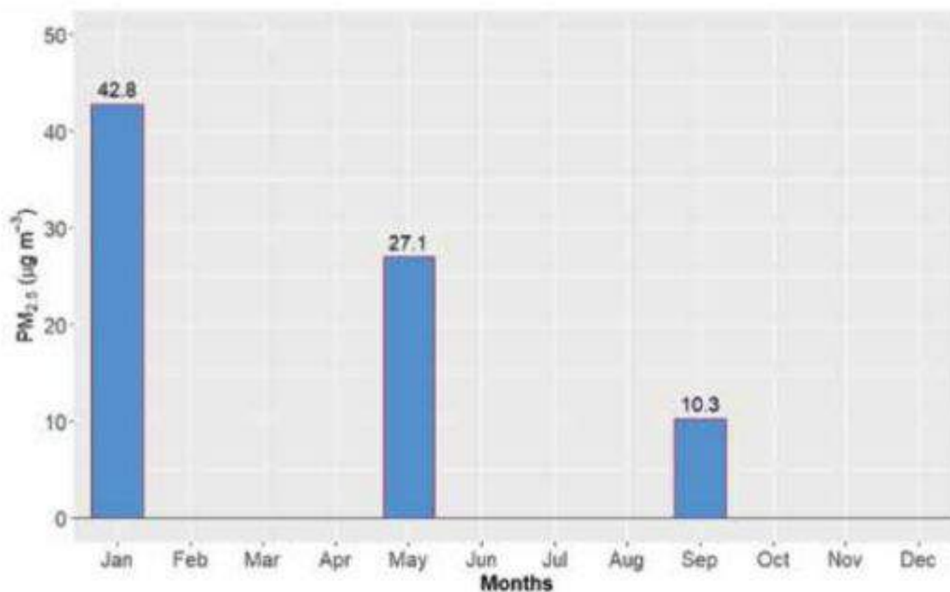
Figure 155: Monthly average of PM 2.5 for Dang Station
