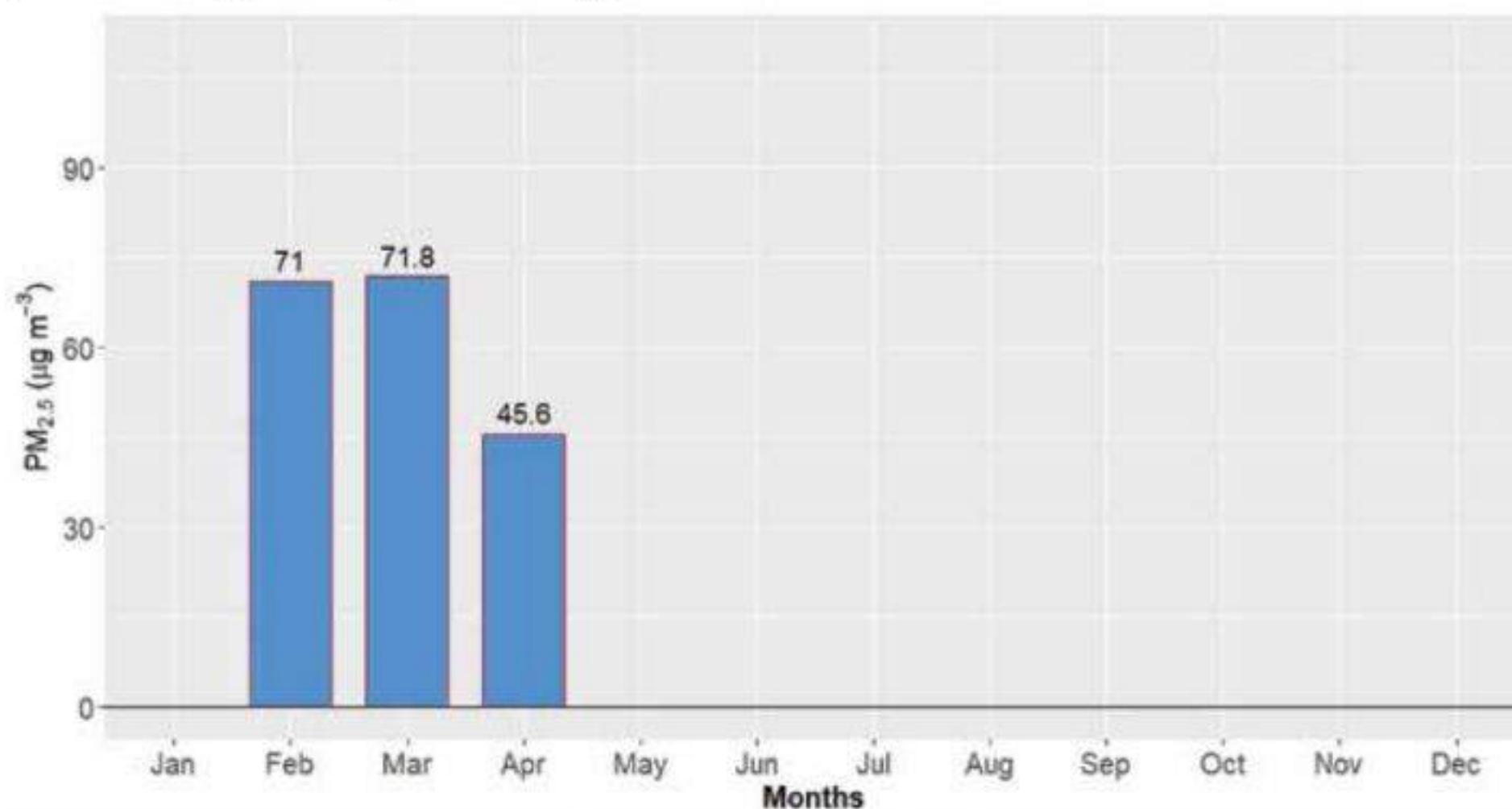
Figure 30: Monthly average of PM 2.5 for Bharatpur Station
