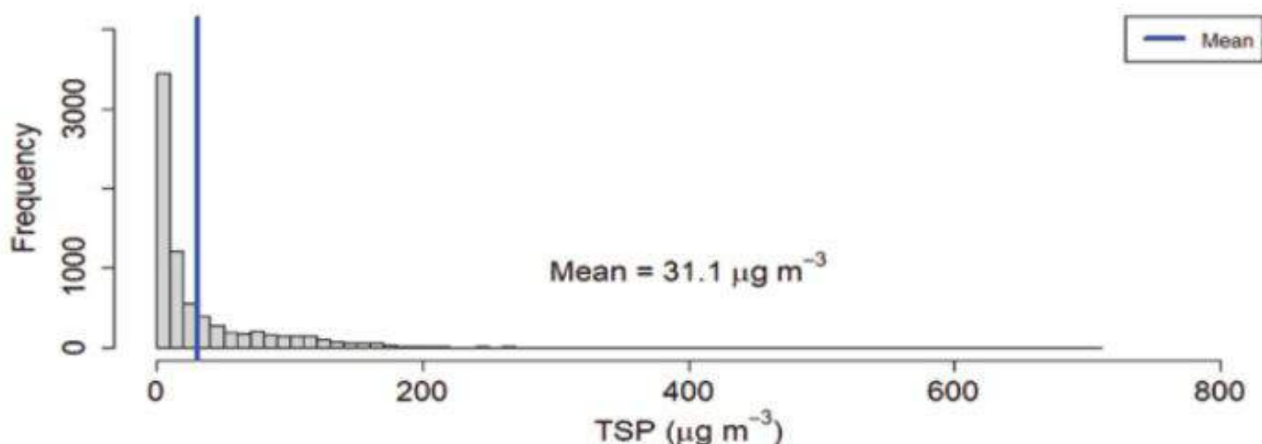
Figure 210: Histogram of TSP for Rara Station
