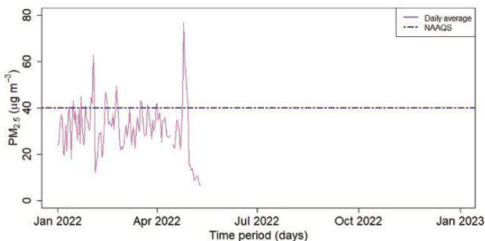
Figure 220: Daily average of PM_{2.5} for Surkhet Station
