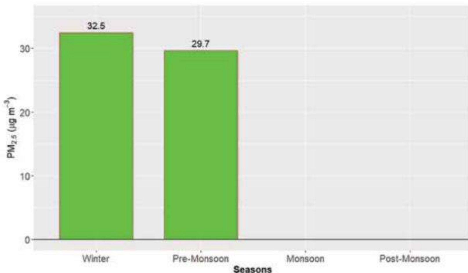
Figure 222: Seasonal average of PM 2.5 for Surkhet Station
