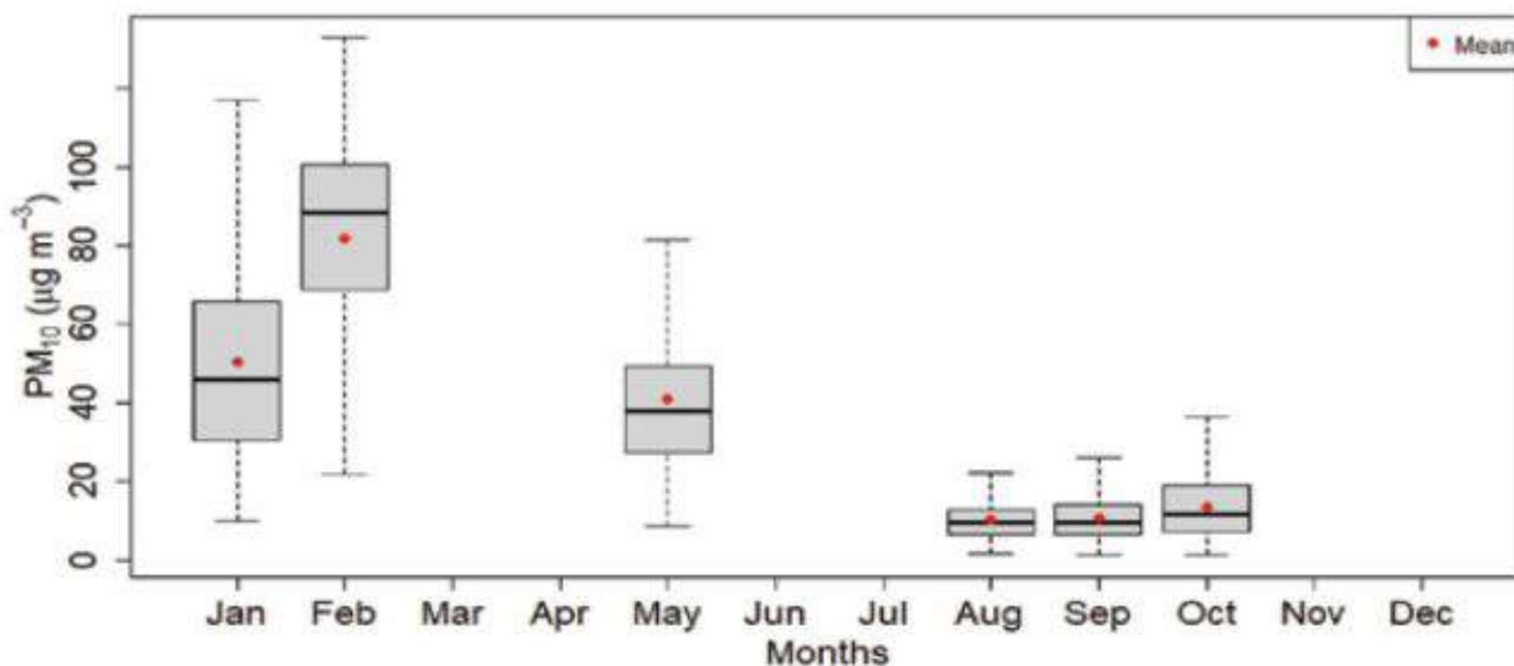
Figure 161: Monthly variation of PM 10 for Dang Station
