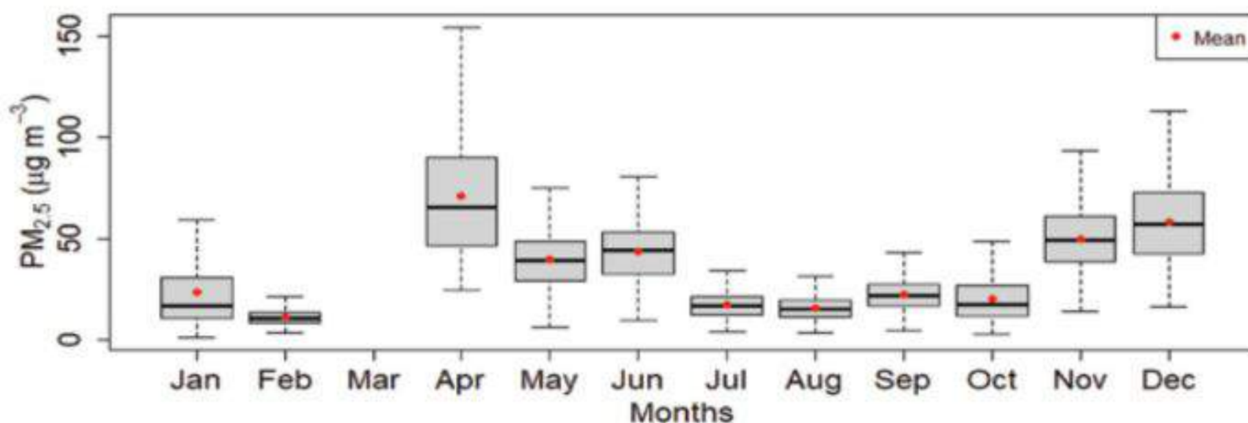
Figure 87: Monthly variation of PM 2.5 for Ratnapark Station
