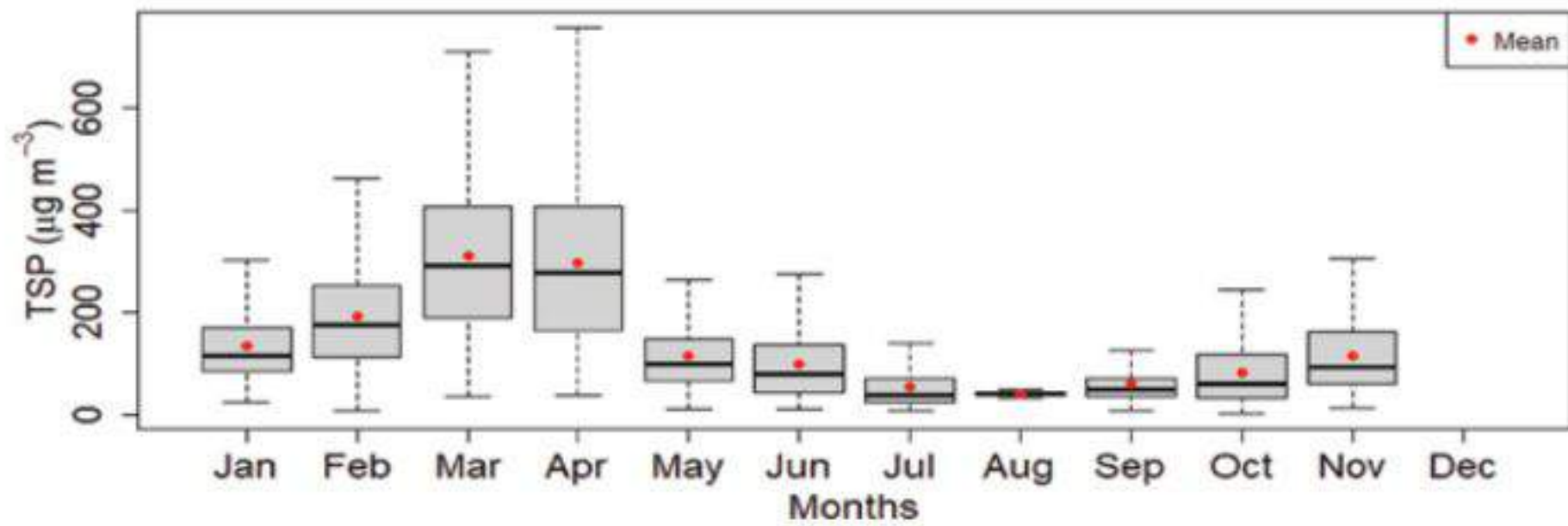
Figure 146: Monthly variation of TSP for Kirtipur Station
