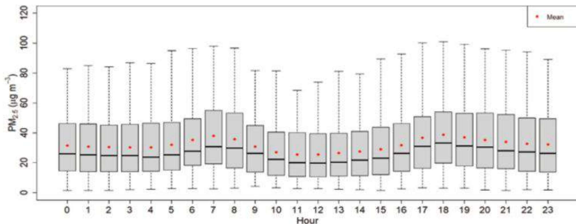
Figure 5: Diurnal variation of PM_{2.5} for Dhankuta Station
