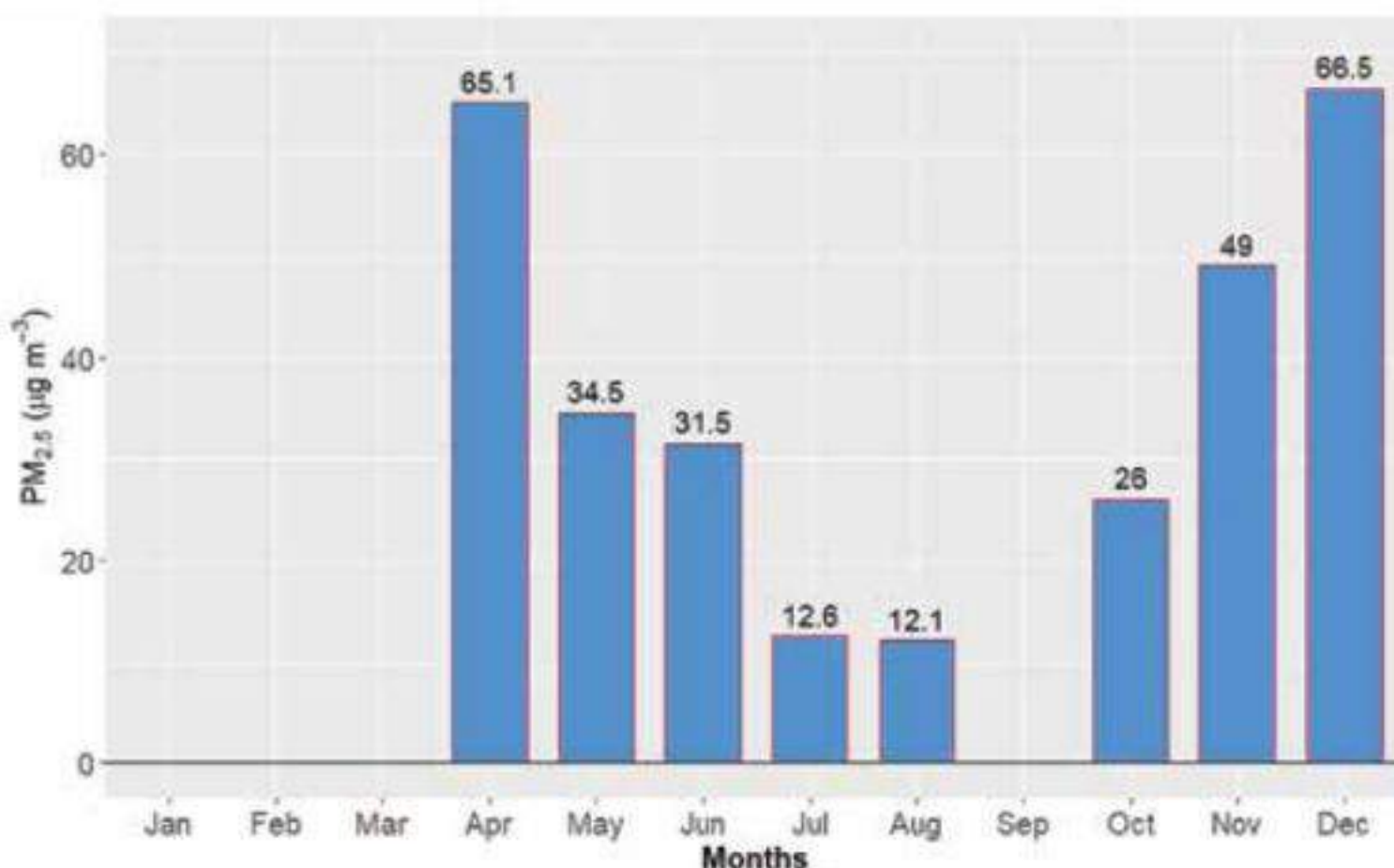
Figure 74: Monthly average of PM 2.5 for Khumaltar Station
