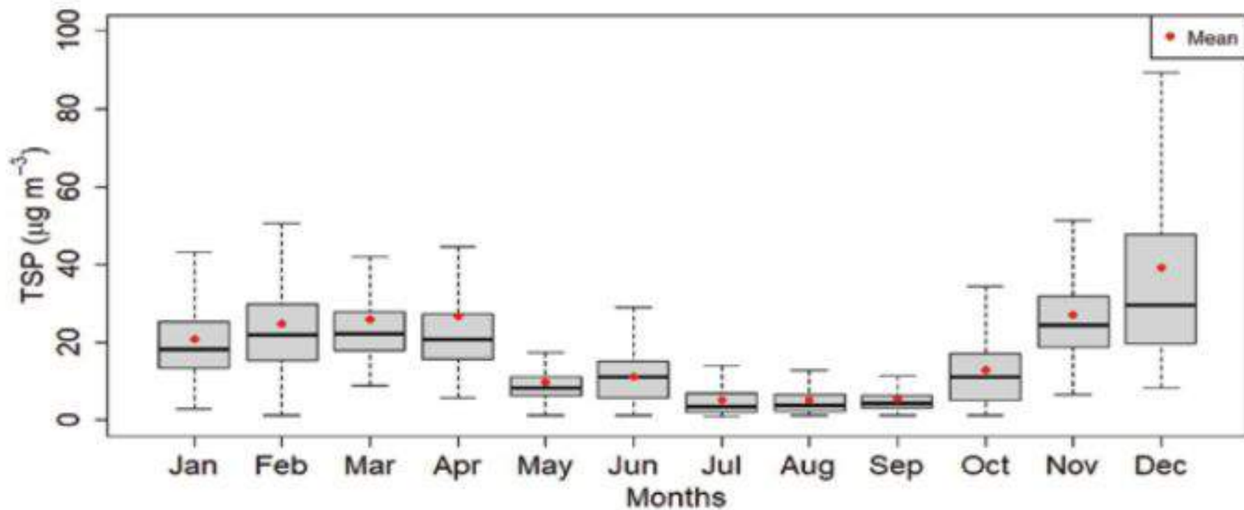
Figure 65: Monthly variation of TSP for Hetauda Station
