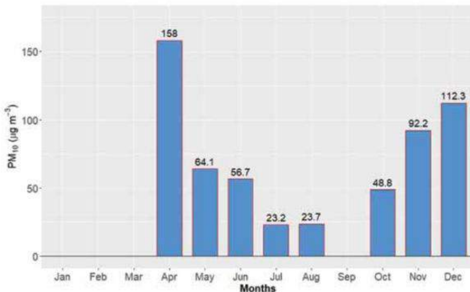
Figure 82: Monthly average of PM 10 for Khumaltar Station
