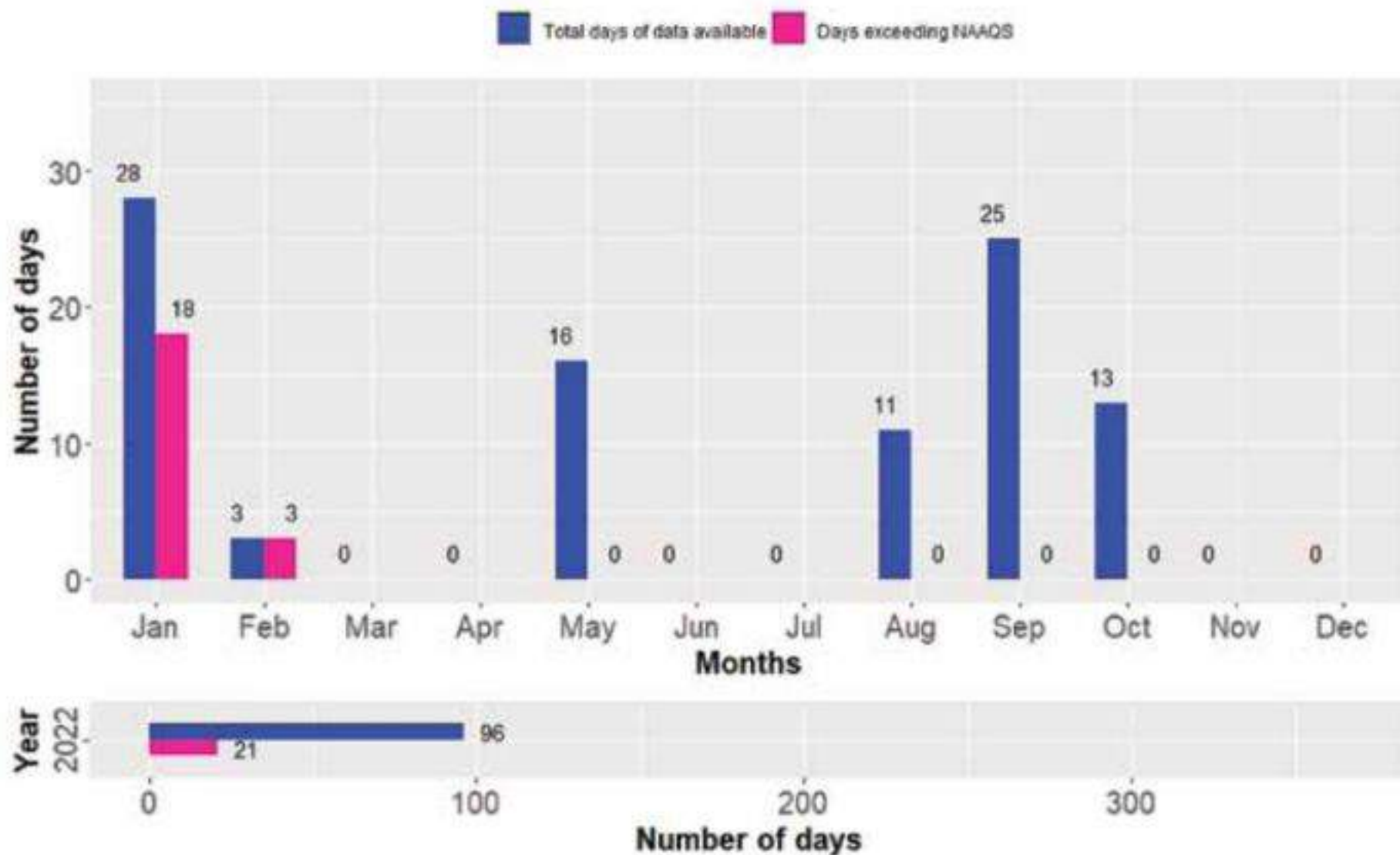
Figure 157: Compliance status of PM 2.5 for Dang Station
