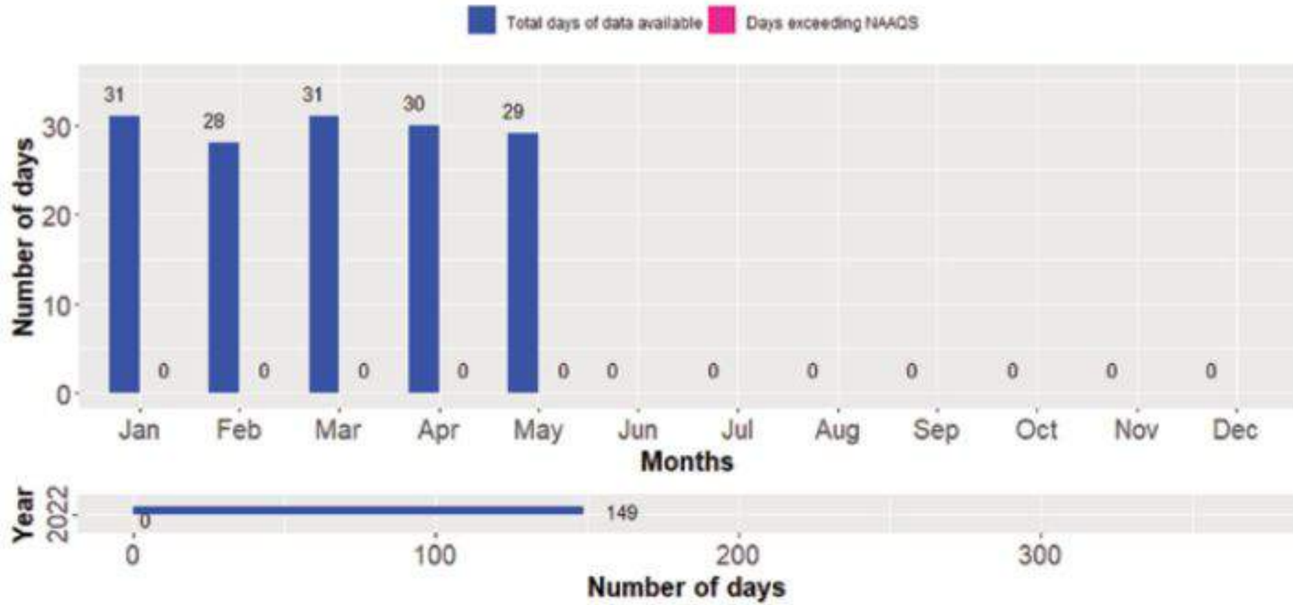
Figure 187: Compliance status of PM 10 for Nepalgunj Station
