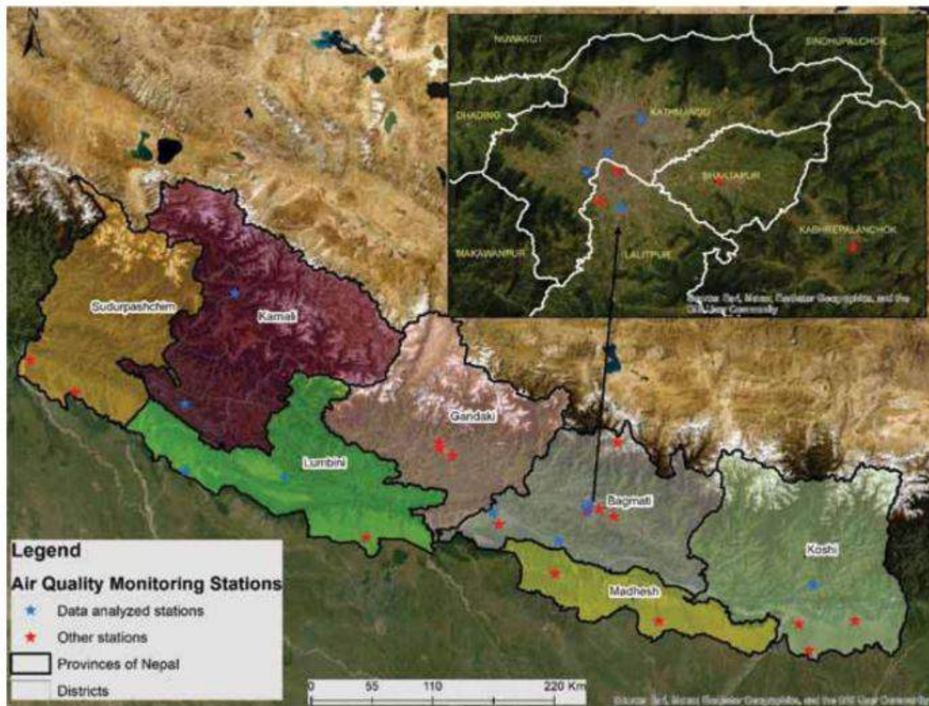
Figure 2: Distribution of AQMS in Nepal
