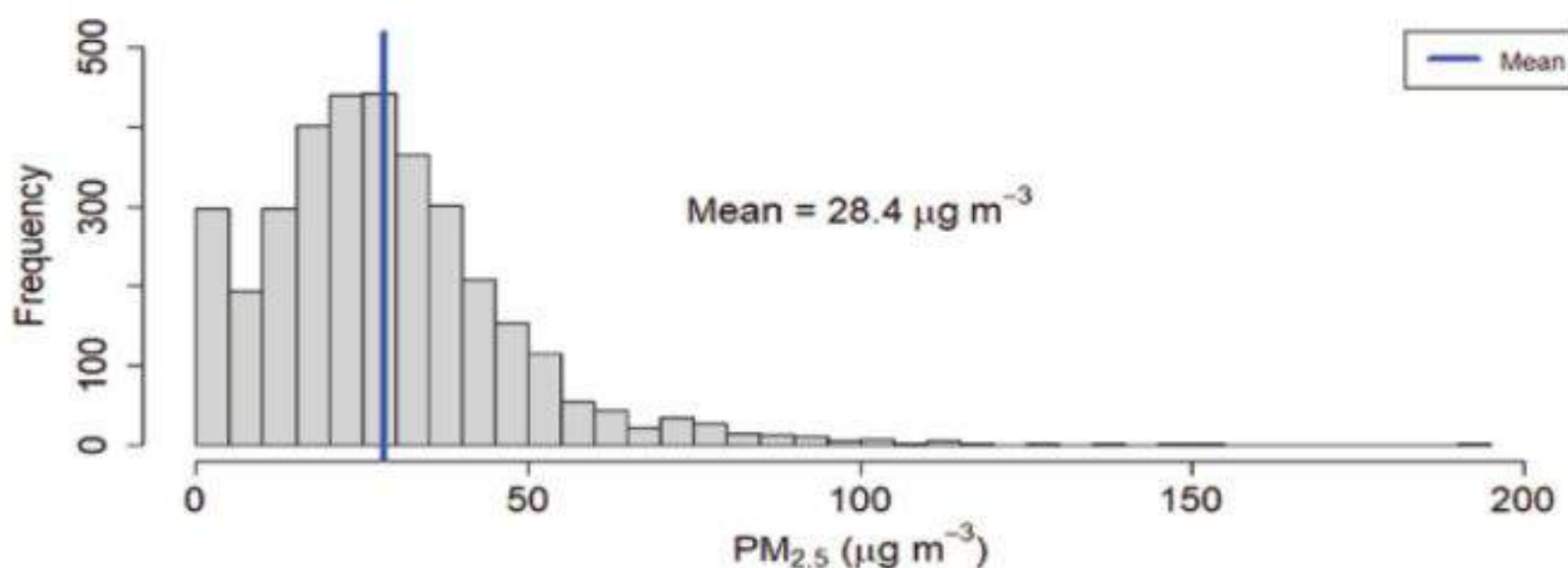
Figure 217: Histogram of PM 2.5 for Surkhet Station
