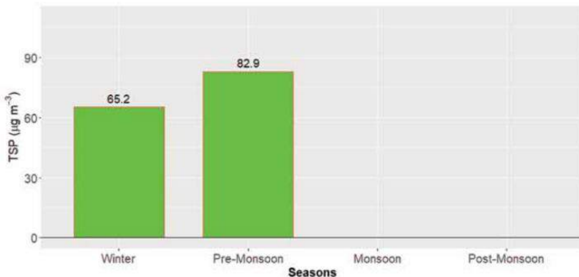
Figure 193: Seasonal average of TSP for Nepalgunj Station
