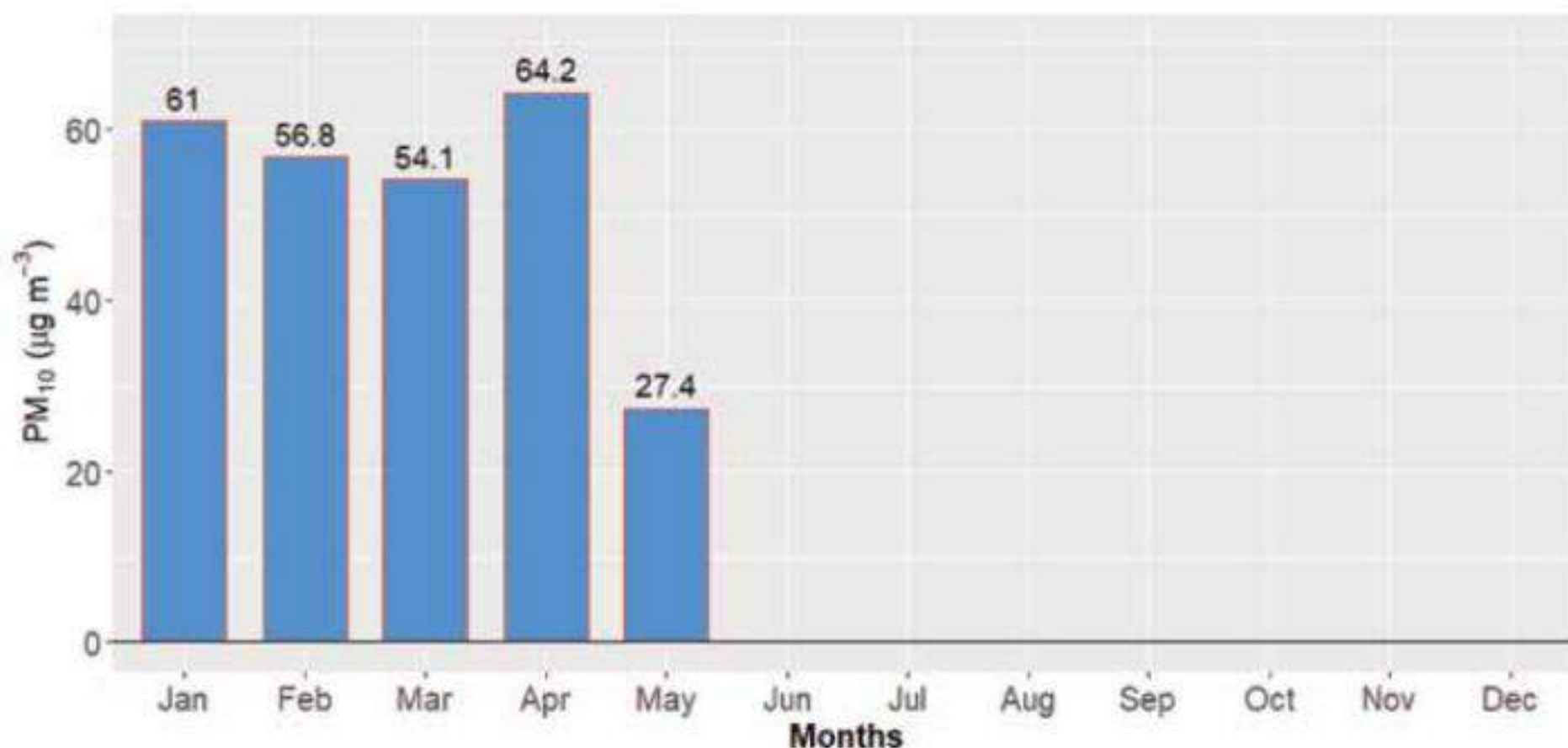
Figure 185: Monthly average of PM 10 for Nepalgunj Station
