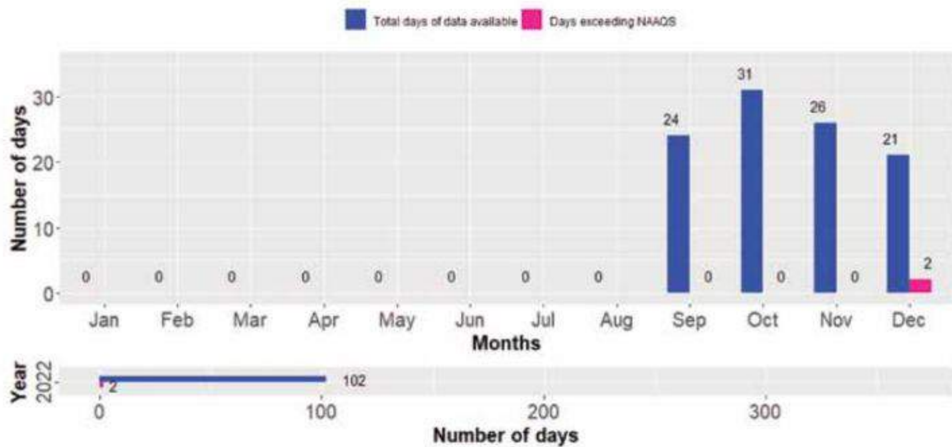
Figure 128: Compliance status of TSP for Shankhapark Station
