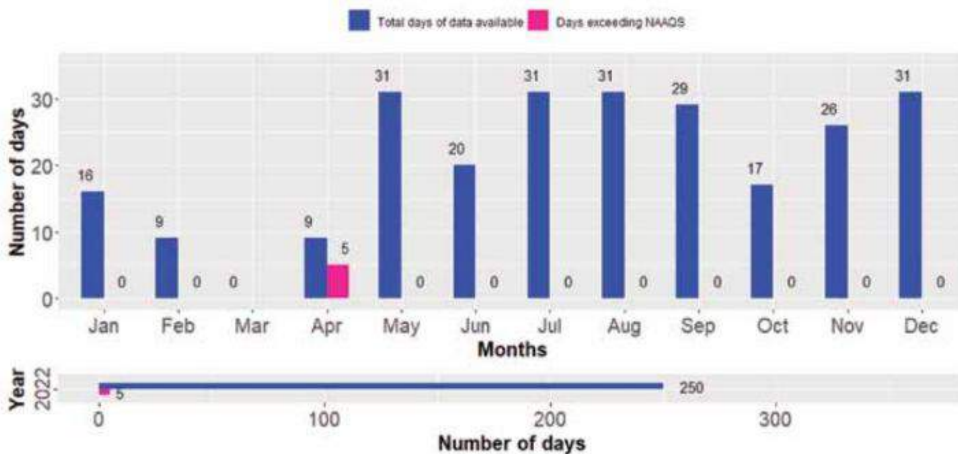
Figure 99: Compliance status of PM 10 for Ratnapark Station
