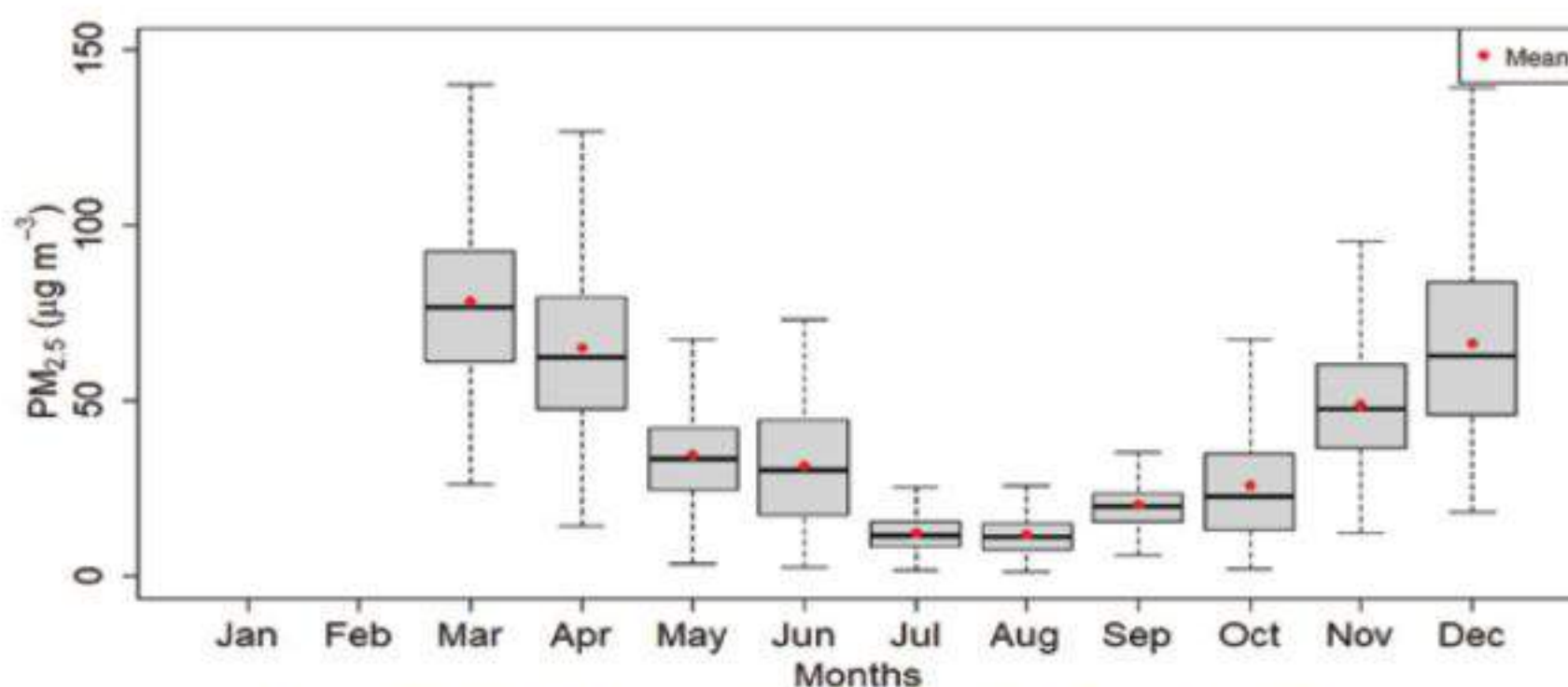
Figure 72: Monthly variation of PM_{2.5} for Khumaltar Station
