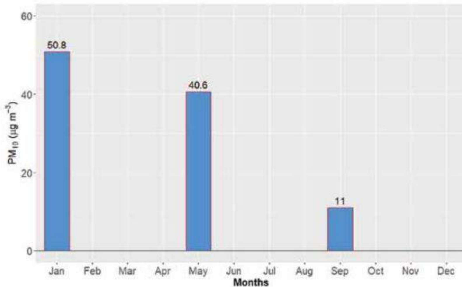
Figure 163: Monthly average of PM_{10} for Dang Station
