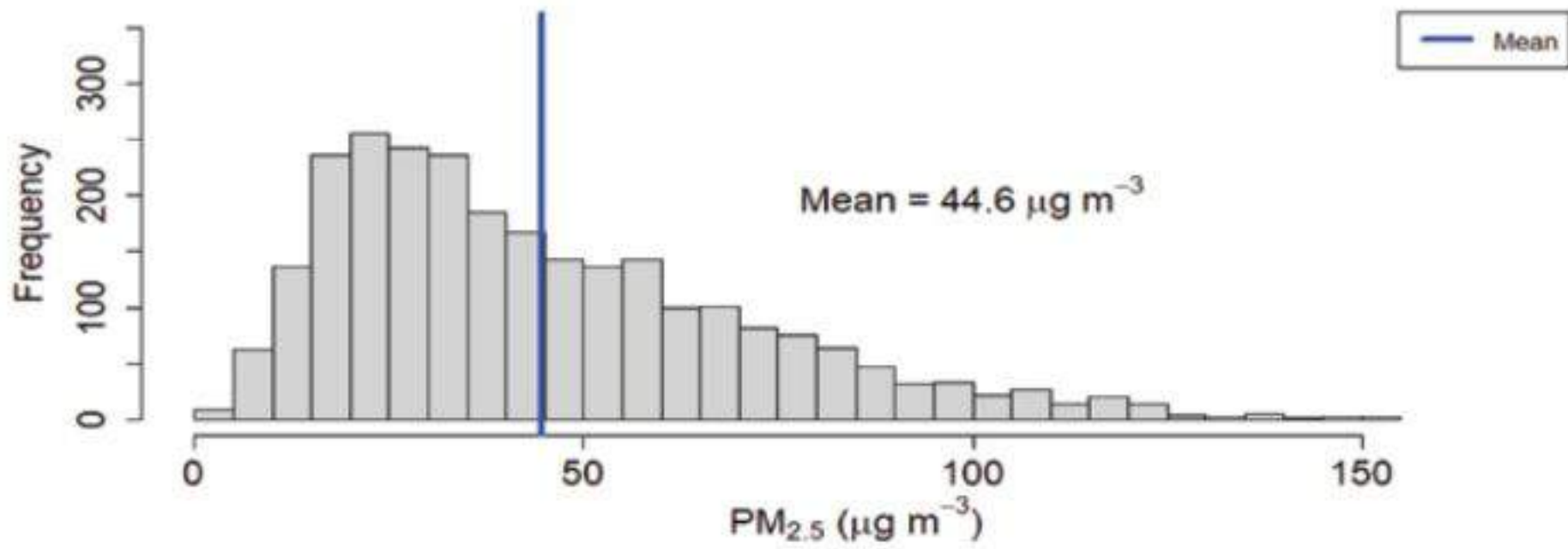
Figure 107: Histogram of PM 2.5 for Shankhapark Station
