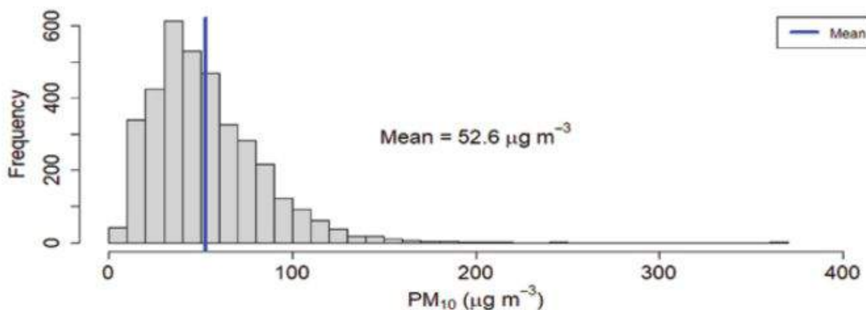
Figure 181: Histogram of PM 10 for Nepalgunj Station
