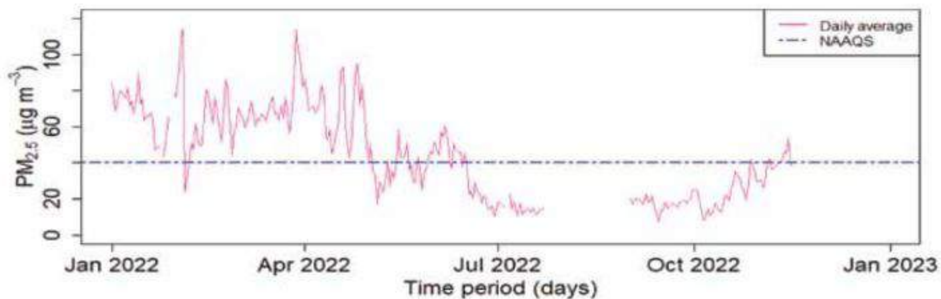
Figure 132: Daily average of PM 2.5 for Kirtipur Station
