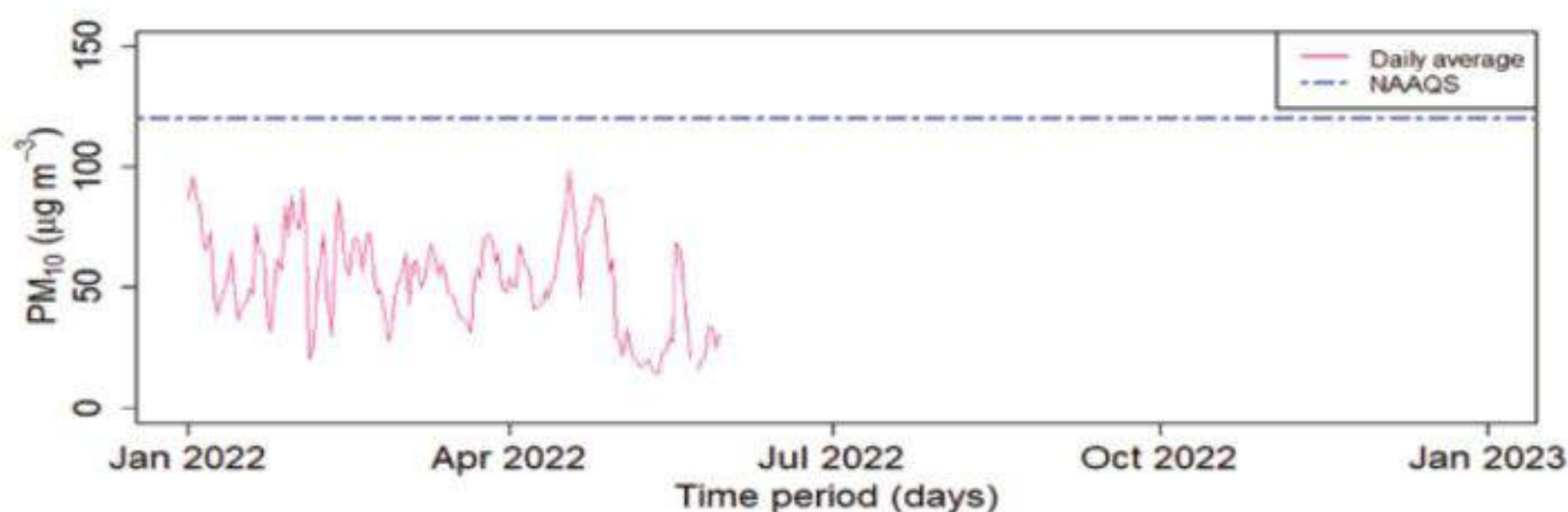
Figure 184: Daily average of PM_{10} for Nepalgunj Station
