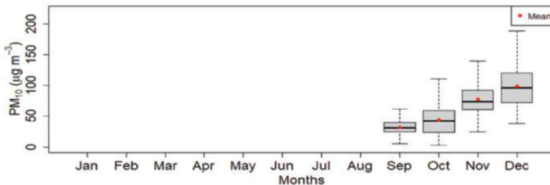
Figure 117: Monthly variation of PM 10 for Shankhapark Station
