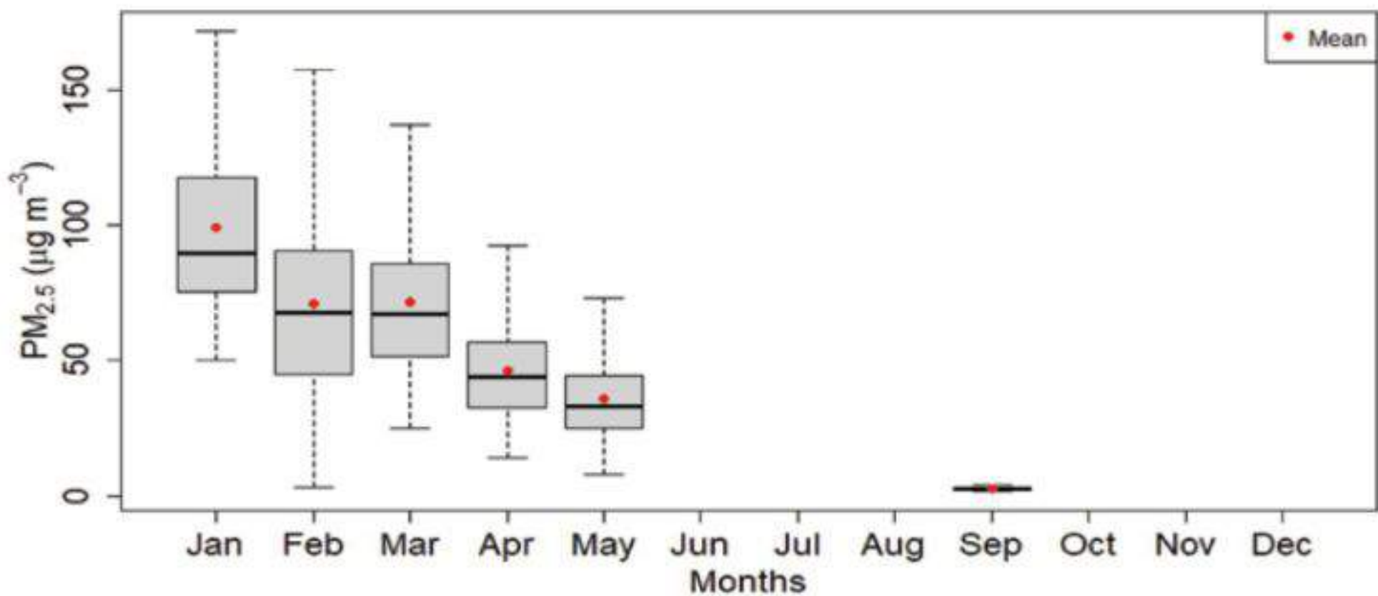
Figure 28: Monthly variation of PM_{2.5} for Bharatpur Station
