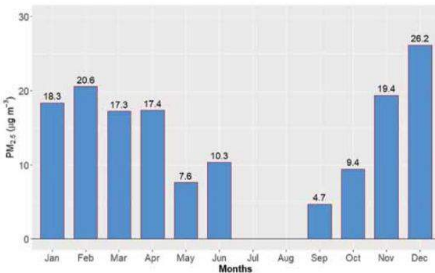
Figure 52: Monthly average of PM 2.5 for Hetauda Station
