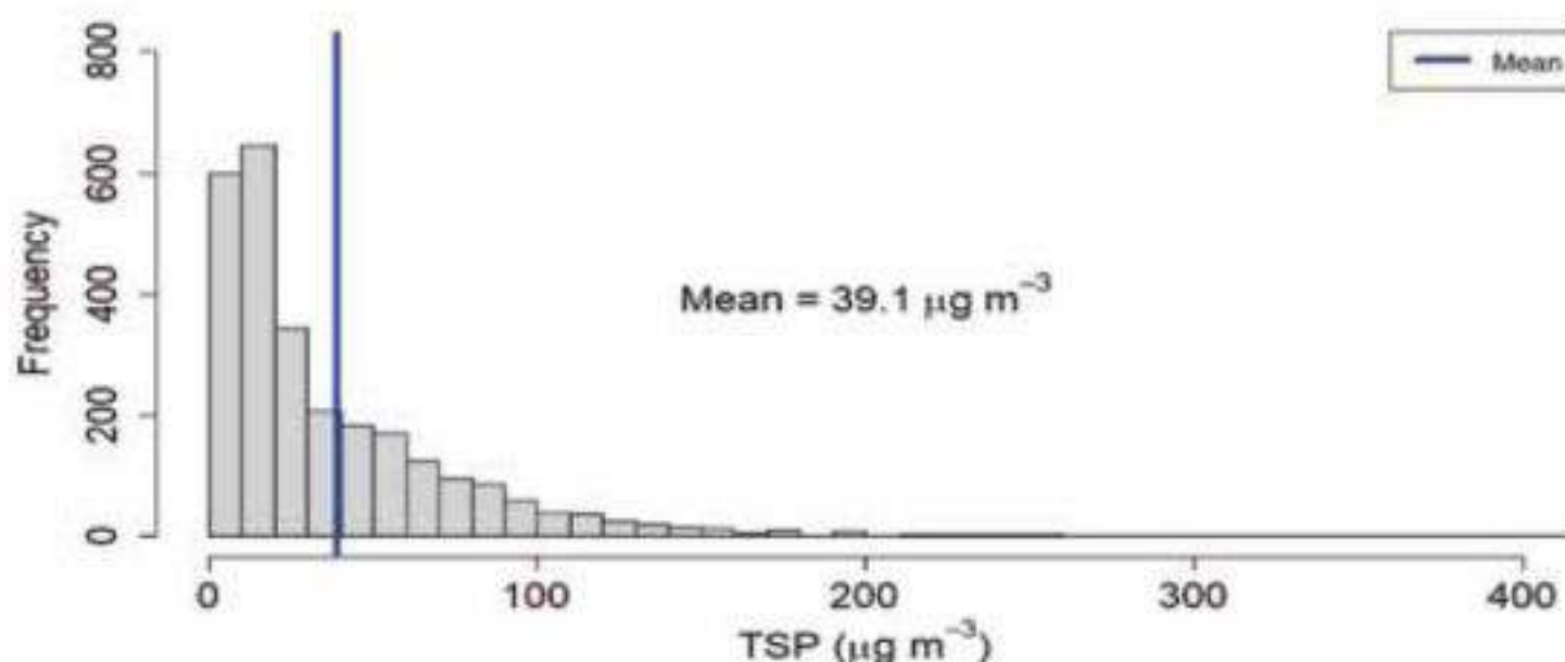
Figure 166: Histogram of TSP for Dang Station
