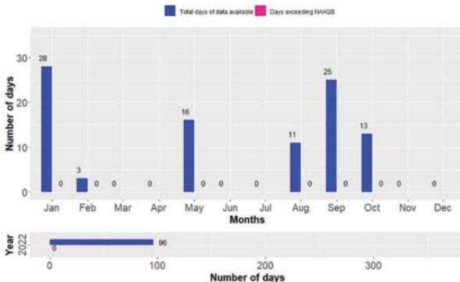
Figure 165: Compliance status of PM 10 for Dang Station
