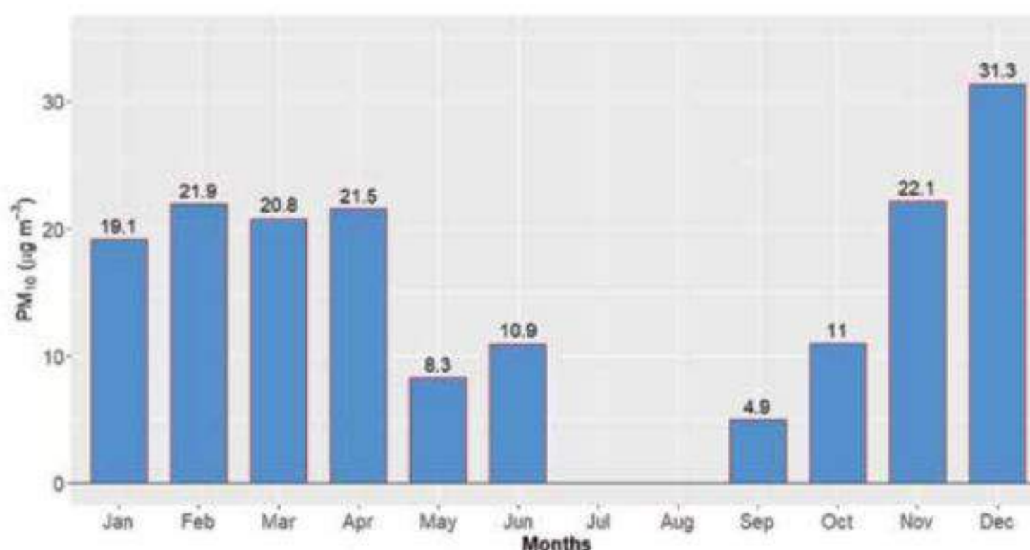
Figure 60: Monthly average of PM 10 for Hetauda Station
