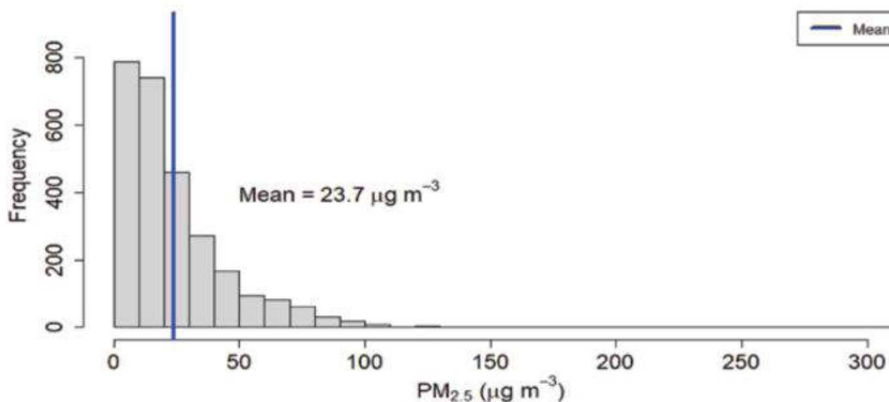
Figure 151: Histogram of PM_{2.5} for Dang Station
