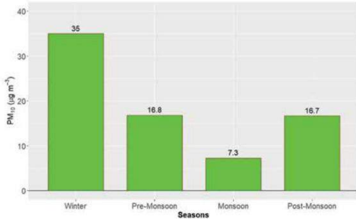
Figure 61: Seasonal average of PM_{10} for Hetauda Station
