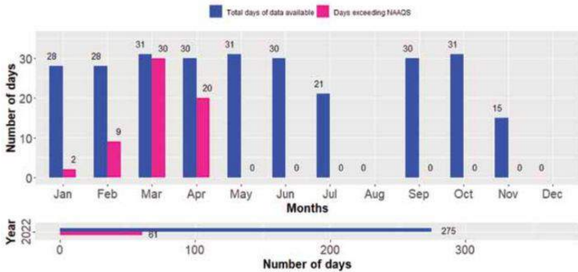
Figure 143: Compliance status of PM 10 for Kirtipur Station
