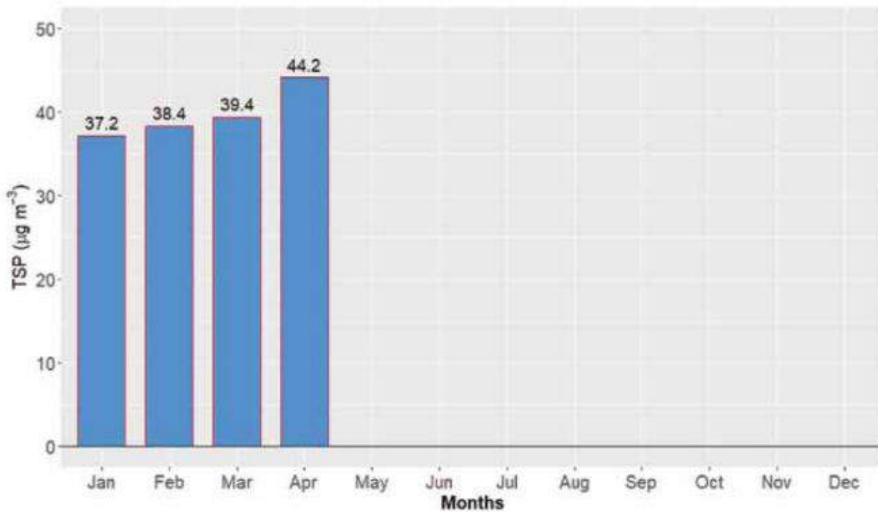
Figure 236: Monthly average of TSP for Surkhet Station
