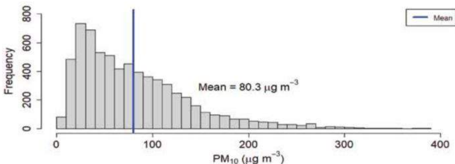
Figure 137: Histogram of PM 10 for Kirtipur Station
