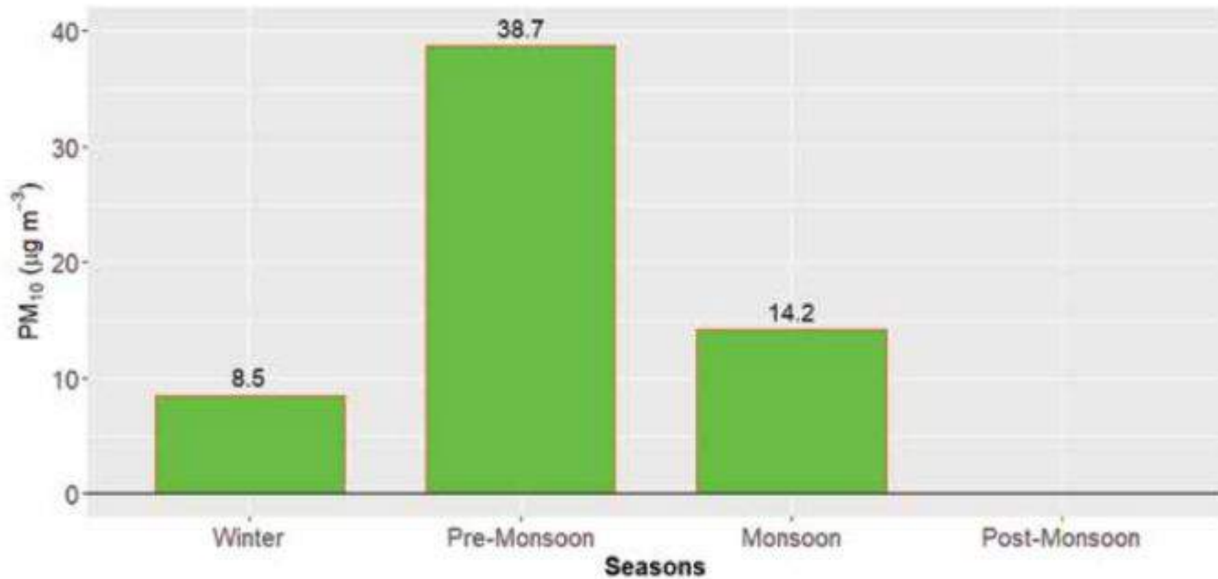
Figure 208: Seasonal average of PM 10 for Rara Station
