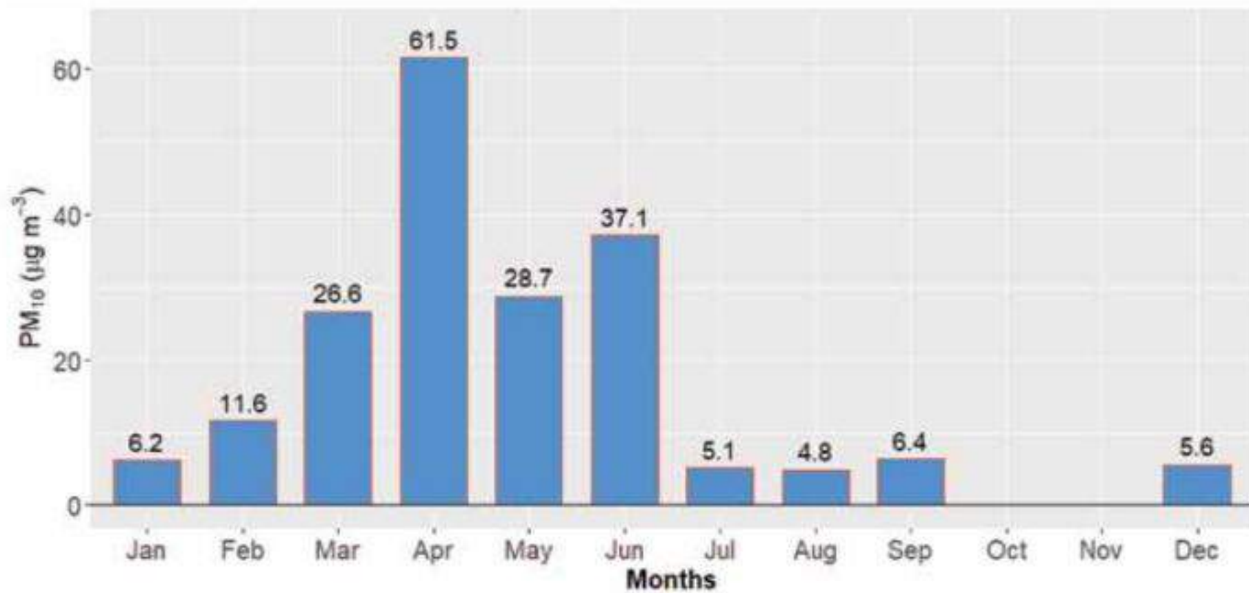
Figure 207: Monthly average of PM 10 for Rara Station
