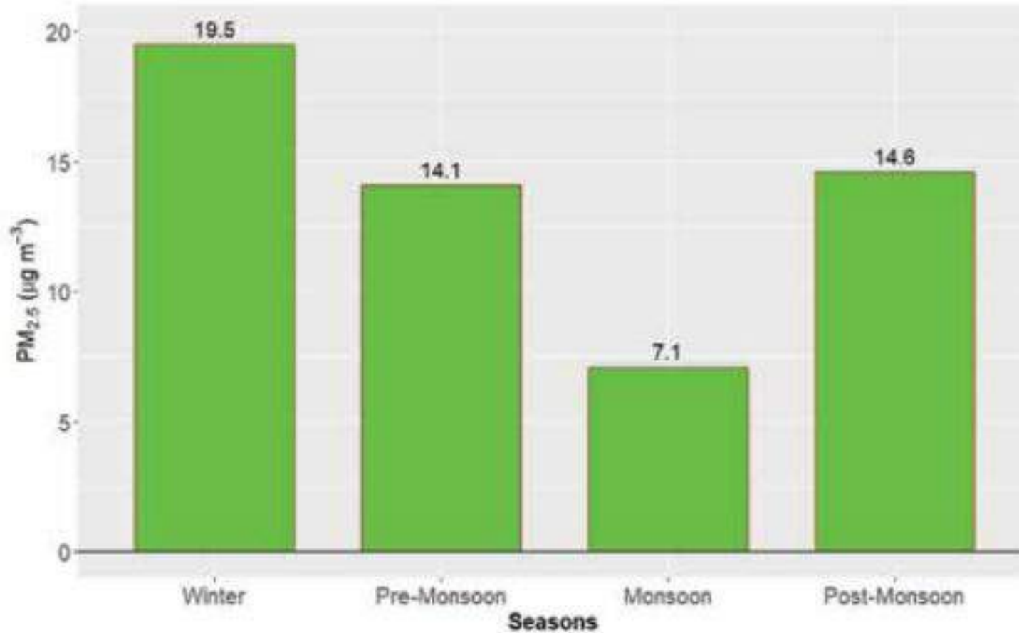
Figure 53: Seasonal average of PM 2.5 for Hetauda Station
