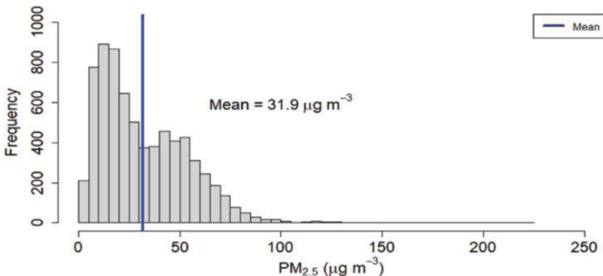
Figure 4: Histogram of PM_{2.5} for Dhankuta Station
