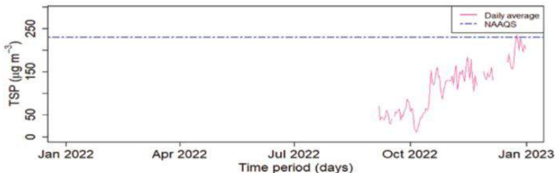
Figure 125: Daily average of TSP for Shankhapark Station
