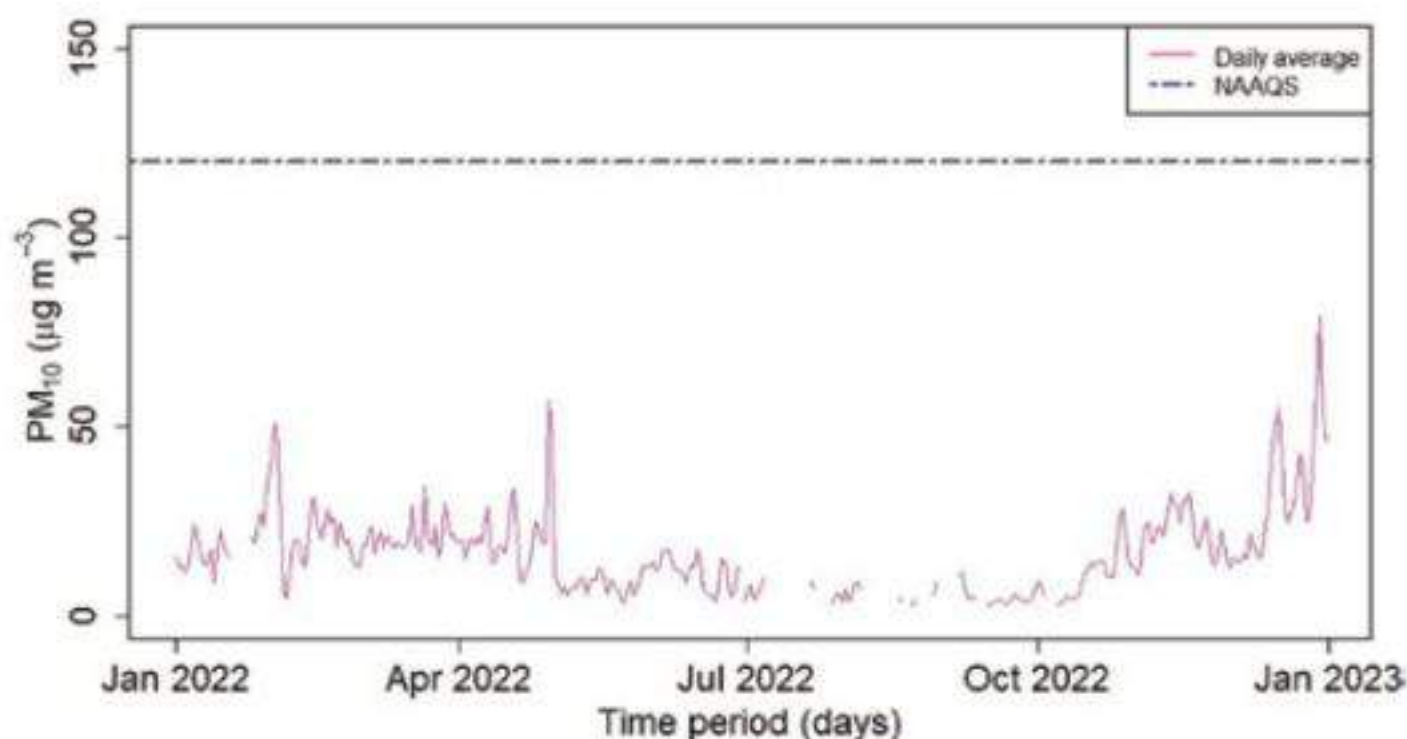
Figure 59: Daily average of PM 10 for Hetauda Station
