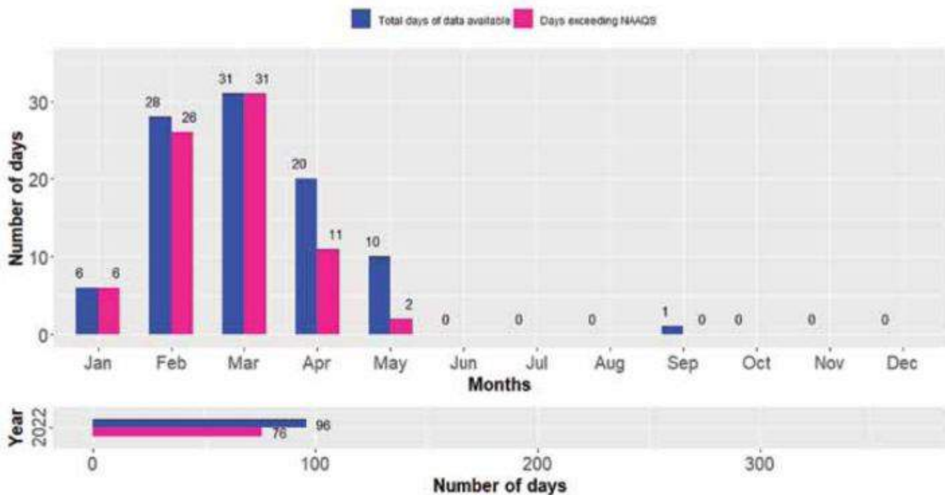
Figure 32: Compliance status of PM 2.5 for Bharatpur Station
