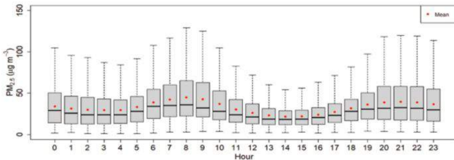
Figure 86: Diurnal variation of PM 2.5 for Ratnapark Station
