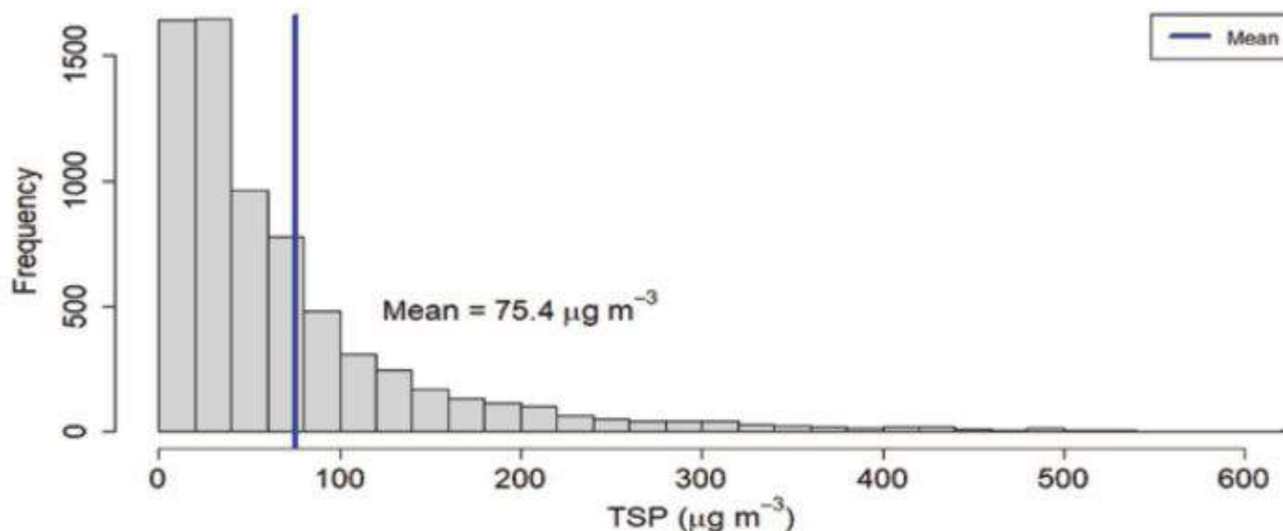
Figure 19: Histogram of TSP for Dhankuta Station
