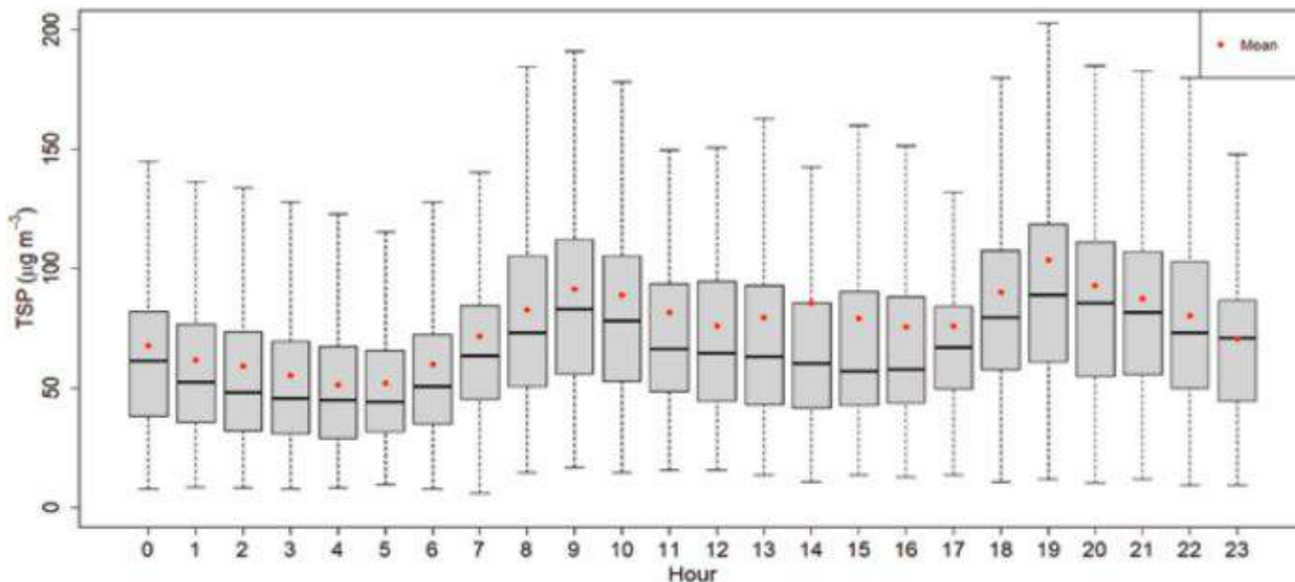
Figure 189: Diurnal variation of TSP for Nepalgunj Station
