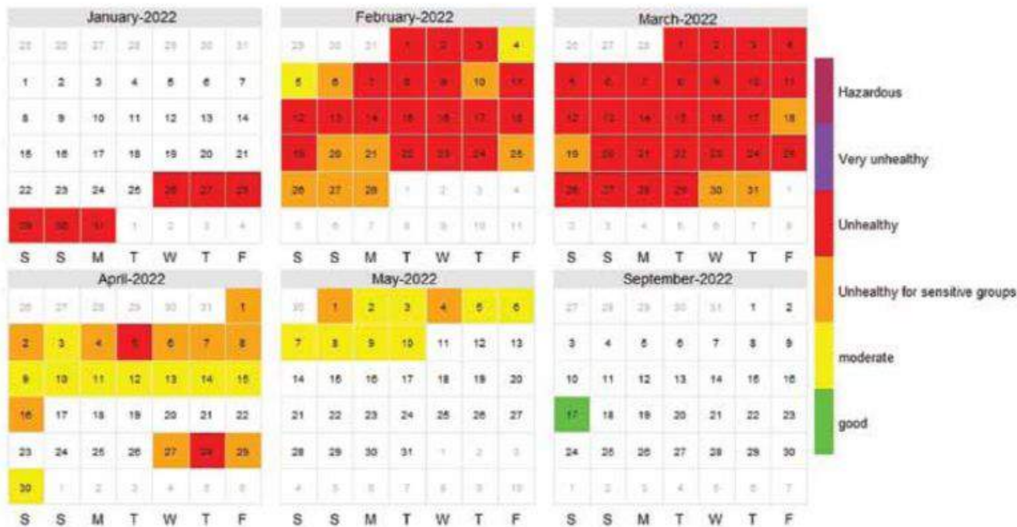
Figure 33: Calendar plot of PM 2.5 for Bharatpur Station
