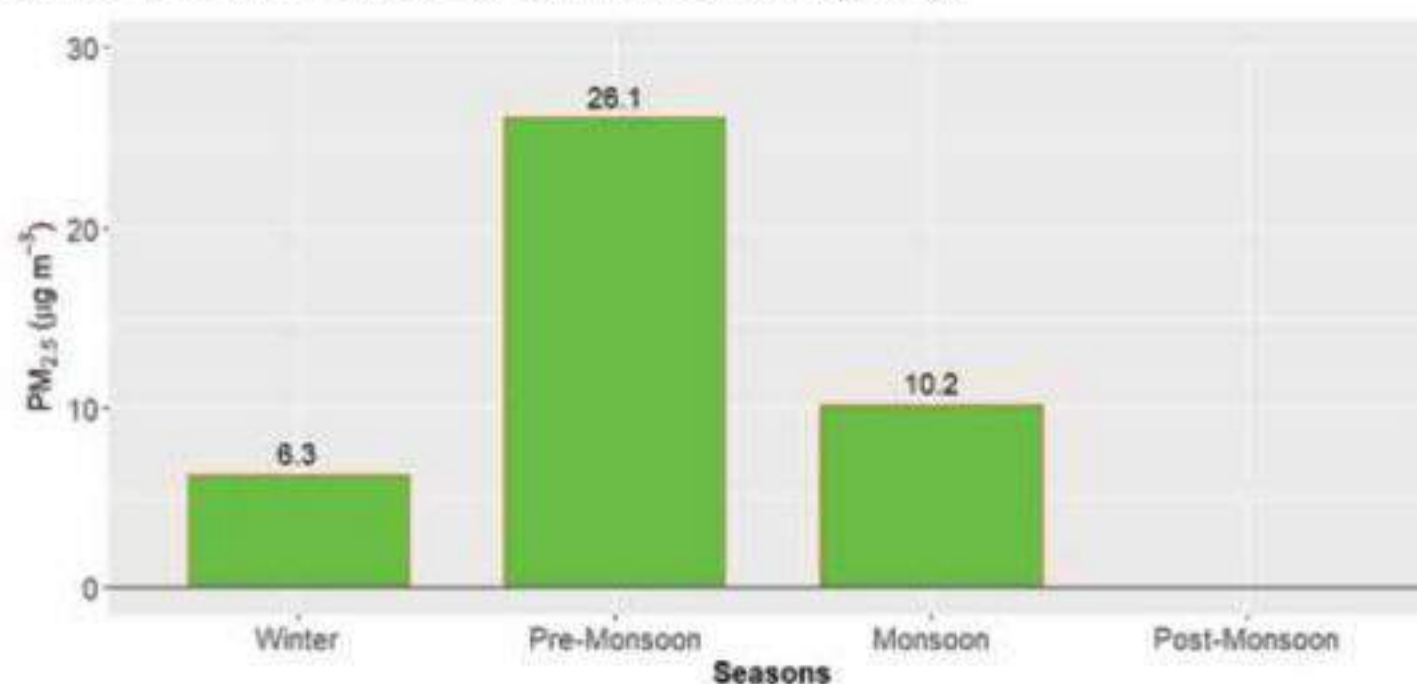
Figure 200: Seasonal average of PM 2.5 for Rara Station
