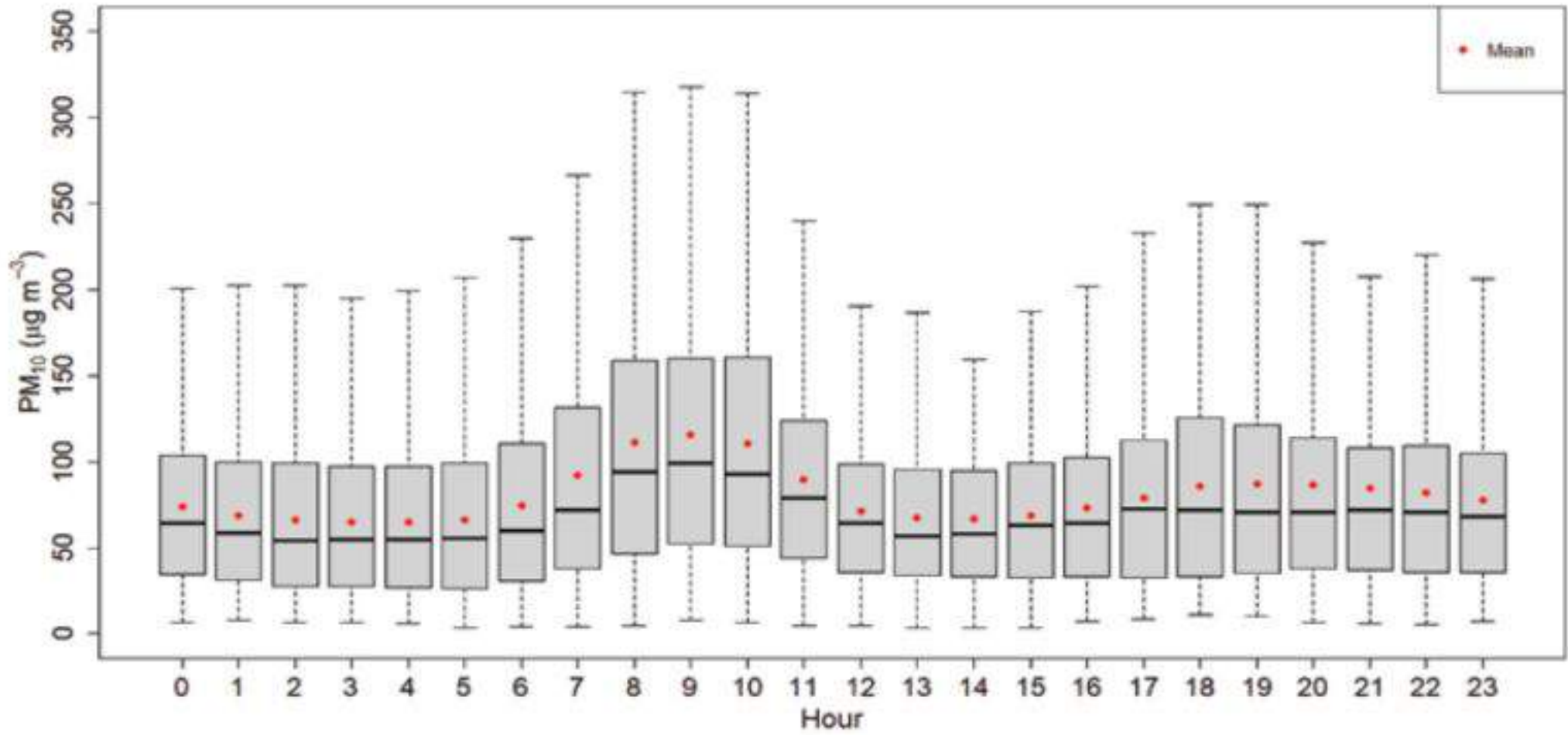
Figure 138: Diurnal variation of PM 10 for Kirtipur Station
