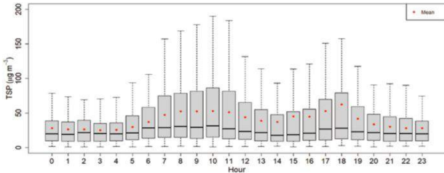
Figure 167: Diurnal variation of TSP for Dang Station
