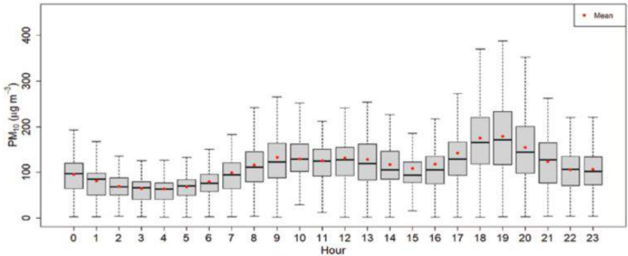
Figure 35: Diurnal variation of PM 10 for Bharatpur Station
