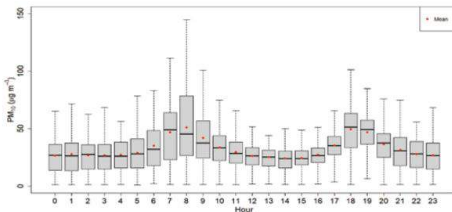
Figure 226: Diurnal variation of PM 10 for Surkhet Station
