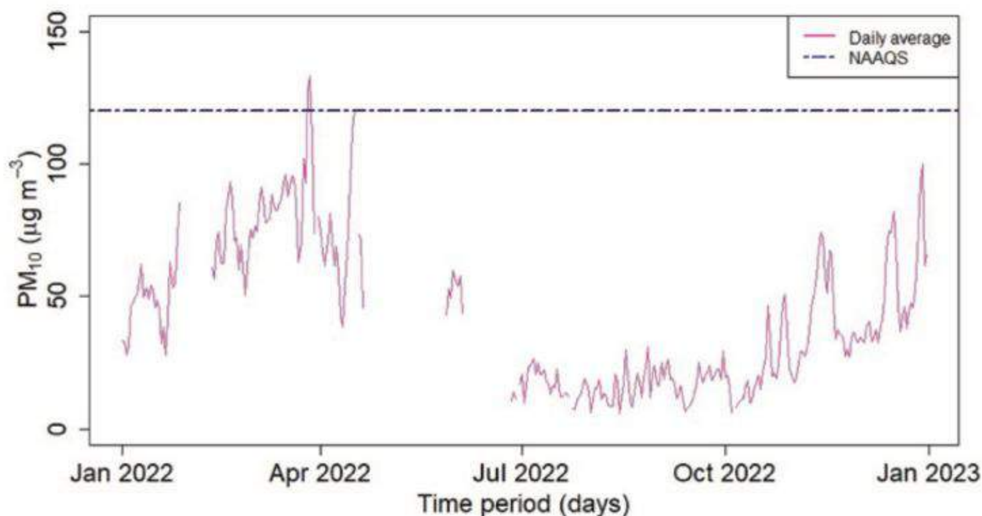
Figure 15: Daily average of PM_{10} for Dhankuta Station
