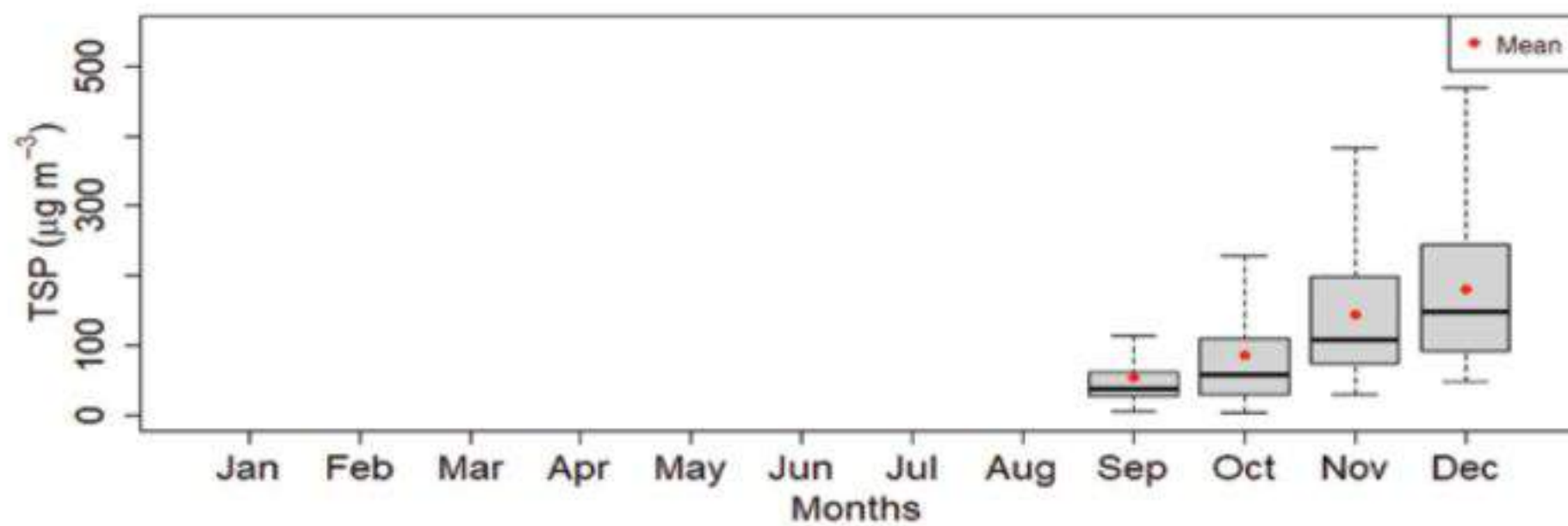
Figure 124: Monthly variation of TSP for Shankhapark Station
