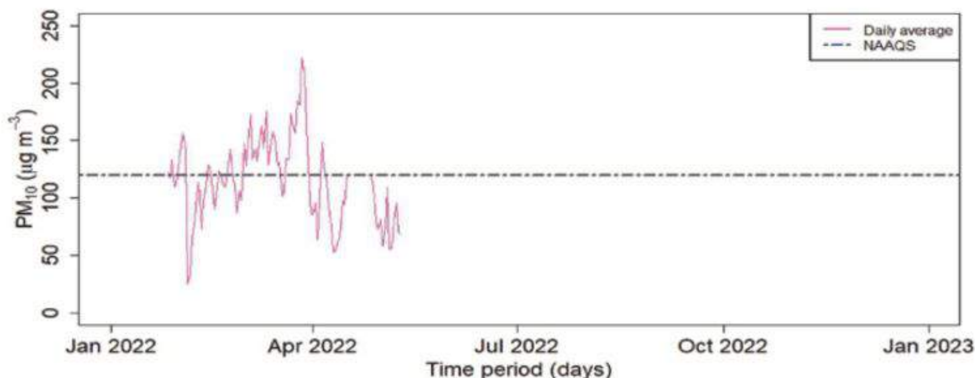
Figure 37: Daily average of PM 10 for Bharatpur Station
