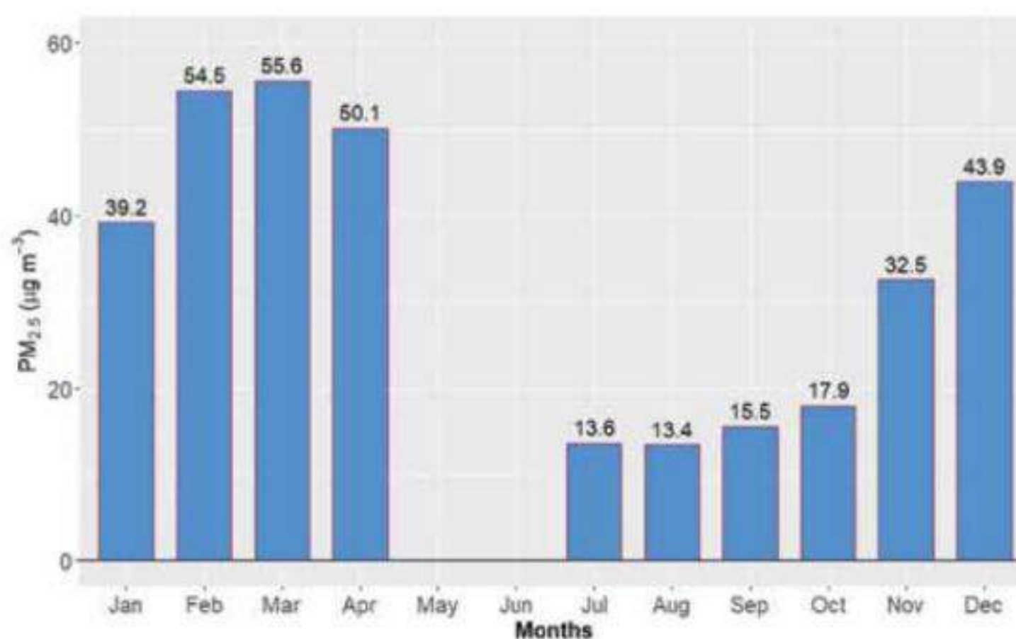
Figure 8: Monthly average of PM 2.5 for Dhankuta Station
