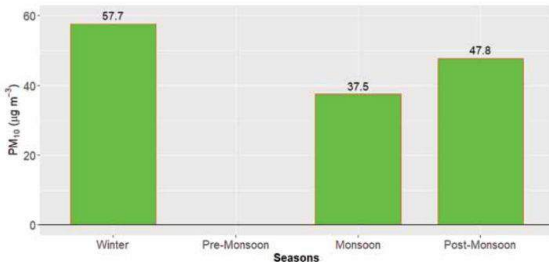
Figure 98: Seasonal average of PM 10 for Ratnapark Station
