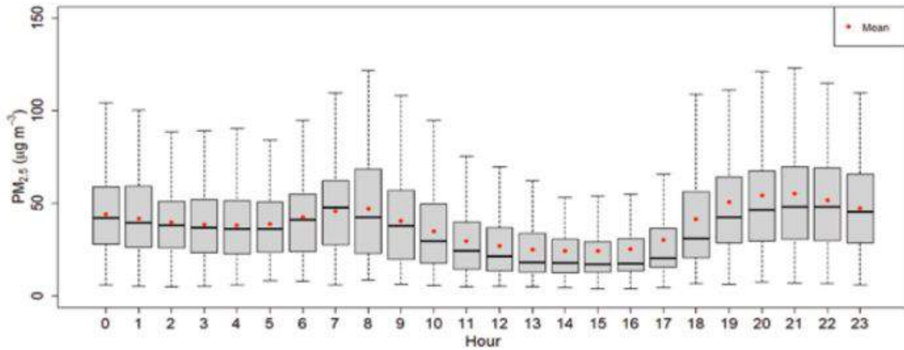
Figure 174: Diurnal variation of PM_{2.5} for Nepalgunj Station
