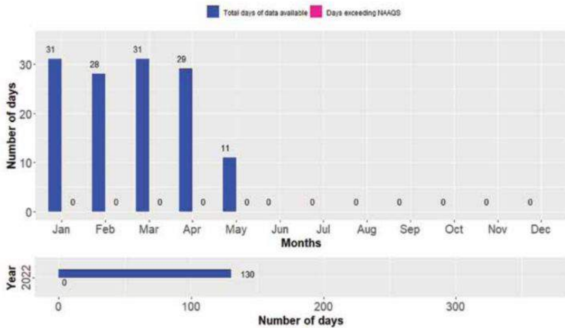
Figure 238: Compliance status of TSP for Surkhet Station
