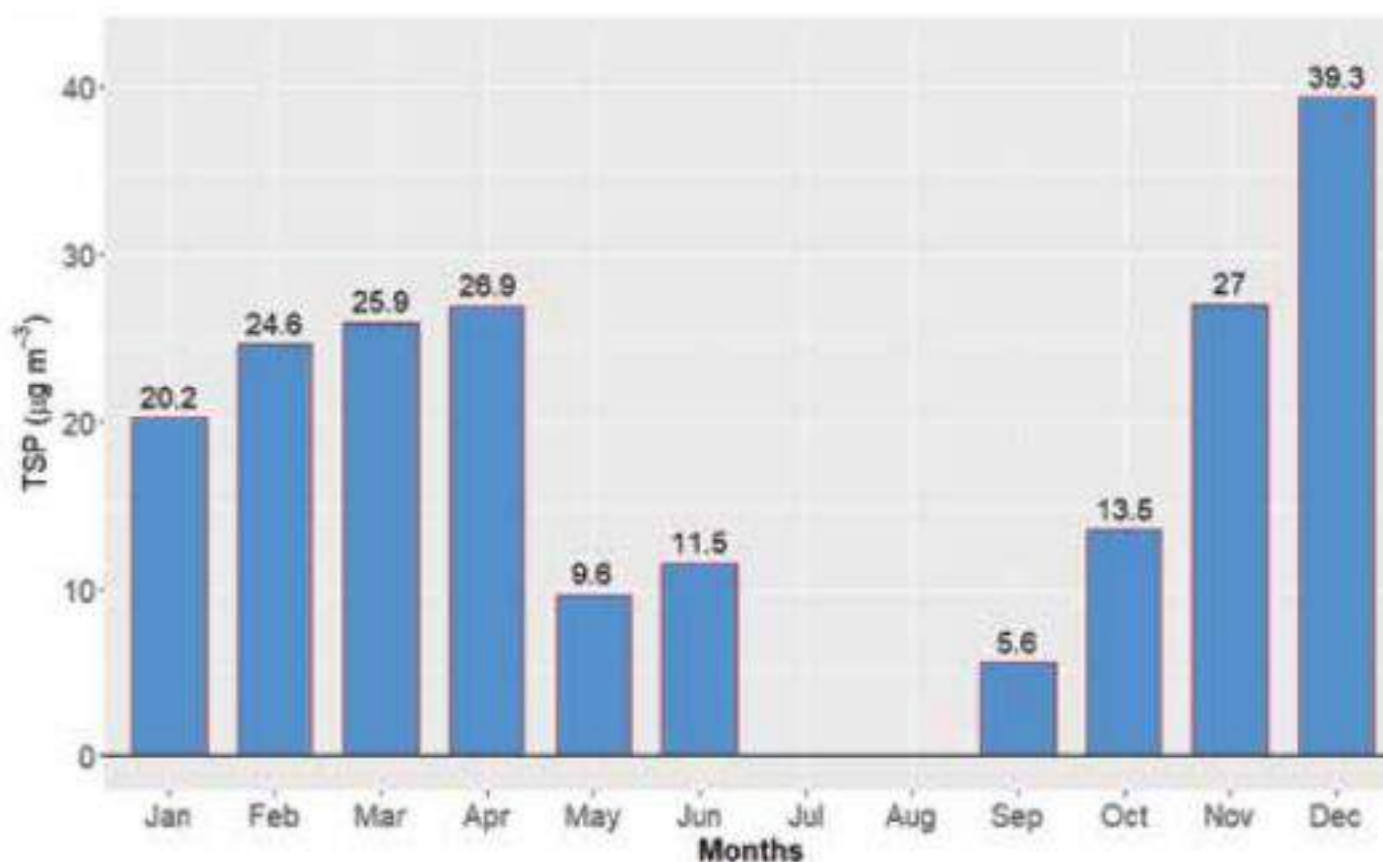
Figure 67: Monthly average of TSP for Hetauda Station
